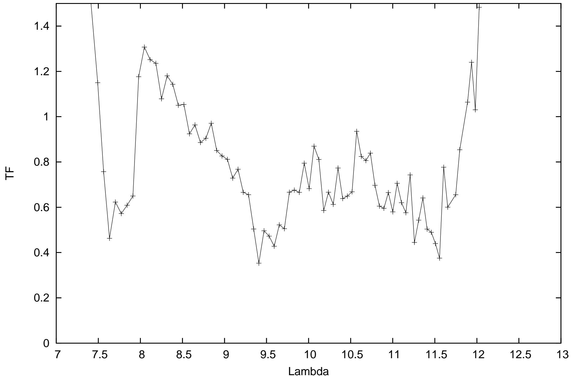
calHD050778_flux0.52_diam3.9_r.MIDI.2009-01-16T05_40_14.015 SCIPHOT
