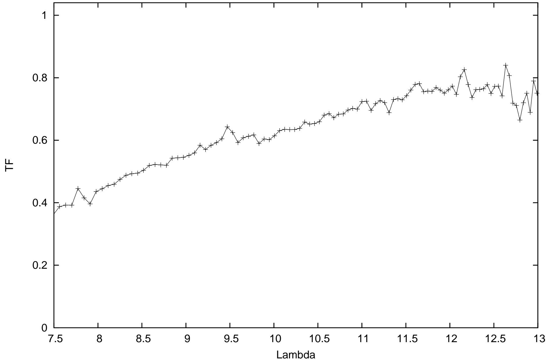
calHD048915_flux-1.39_diam6.09_r.MIDI.2010-02-07T03_26_05.029_G1H0
