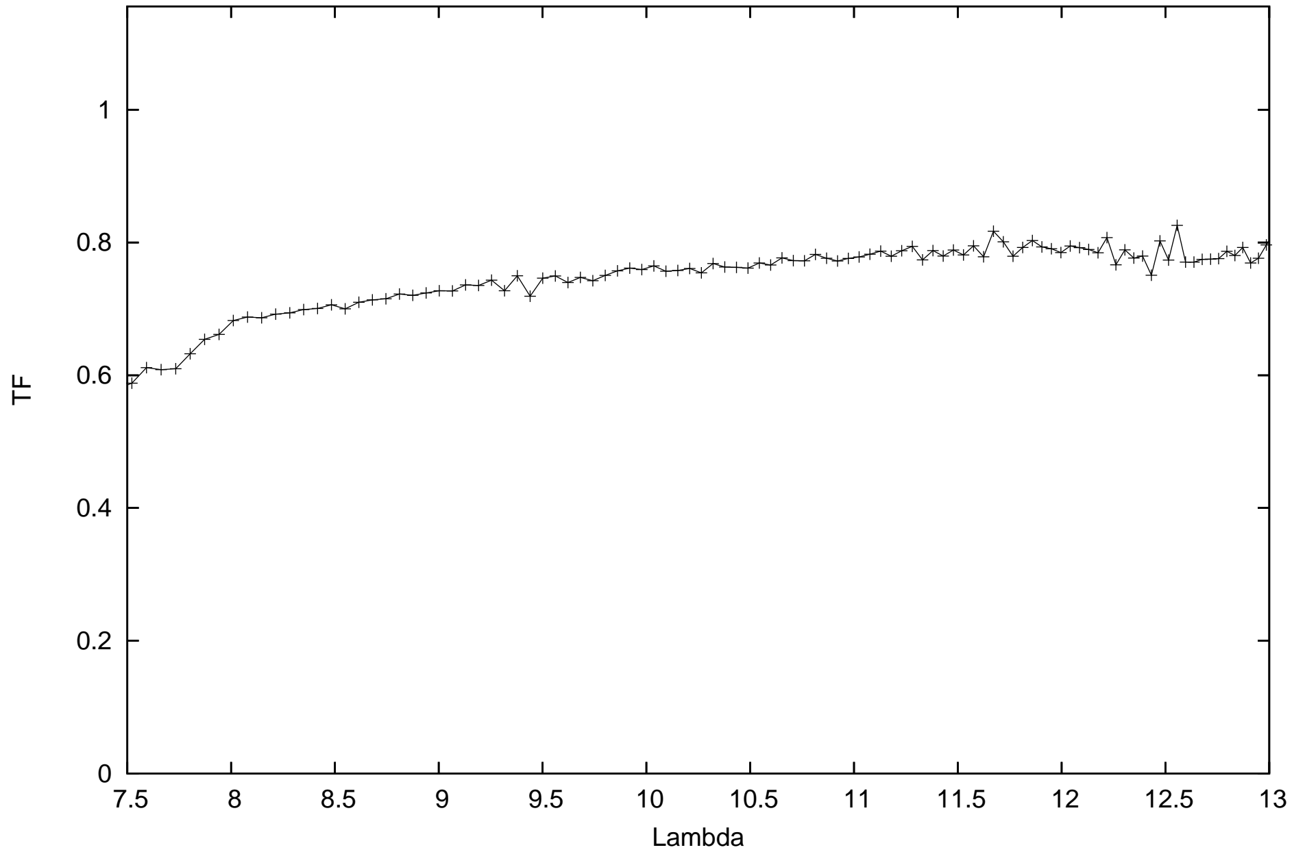
calHD048915_flux-1.39_diam6.09_r.MIDI.2009-11-13T08_47_04.000_E0G0
