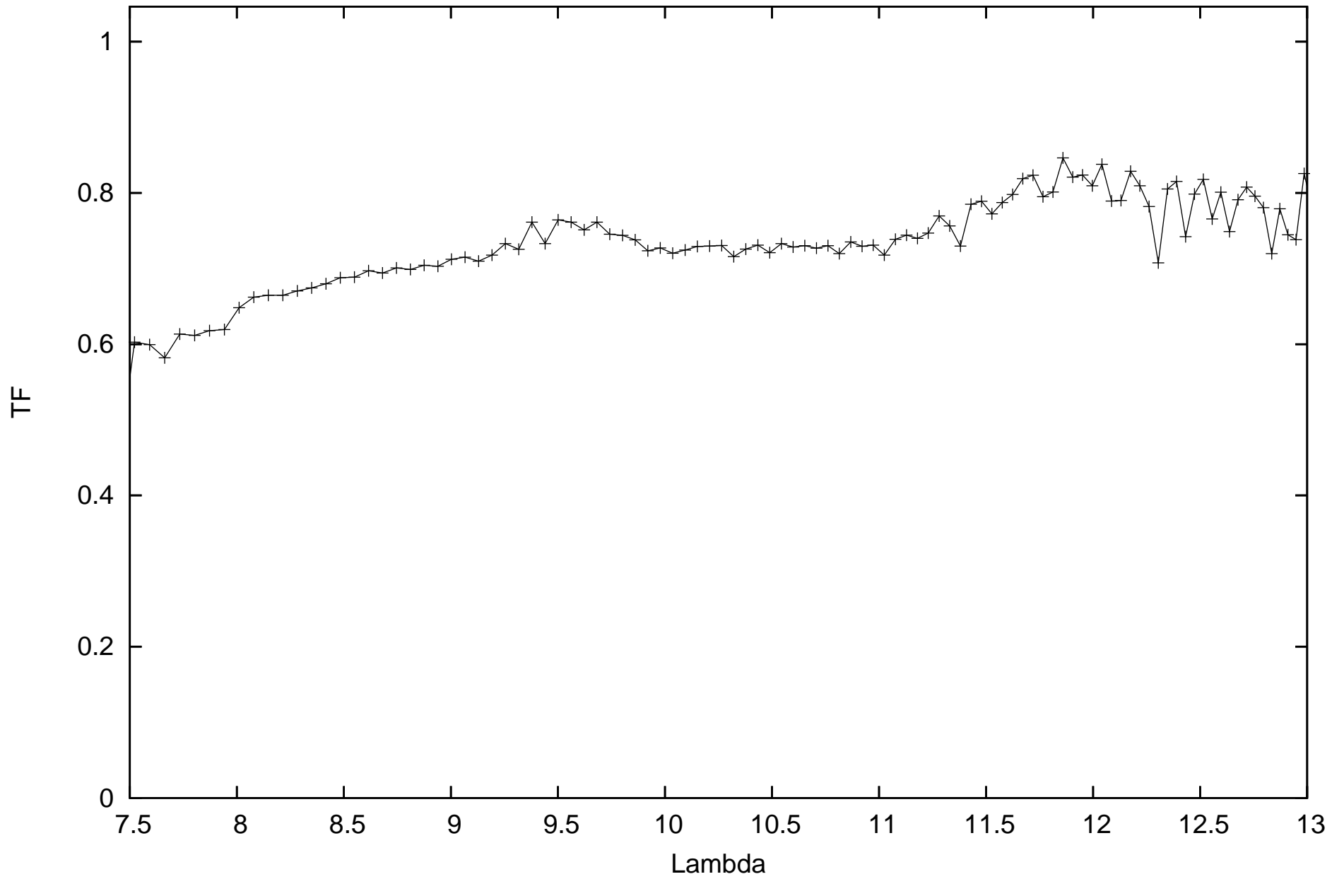
calHD048915_flux-1.39_diam6.09_r.MIDI.2009-01-26T05_07_11.000_HIGHSENS
