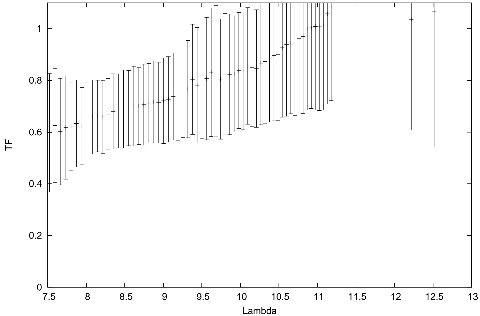
calHD048915_flux-1.39_diam6.09_r.MIDI.2009-01-26T04_07_30.000_HIGHSENS
