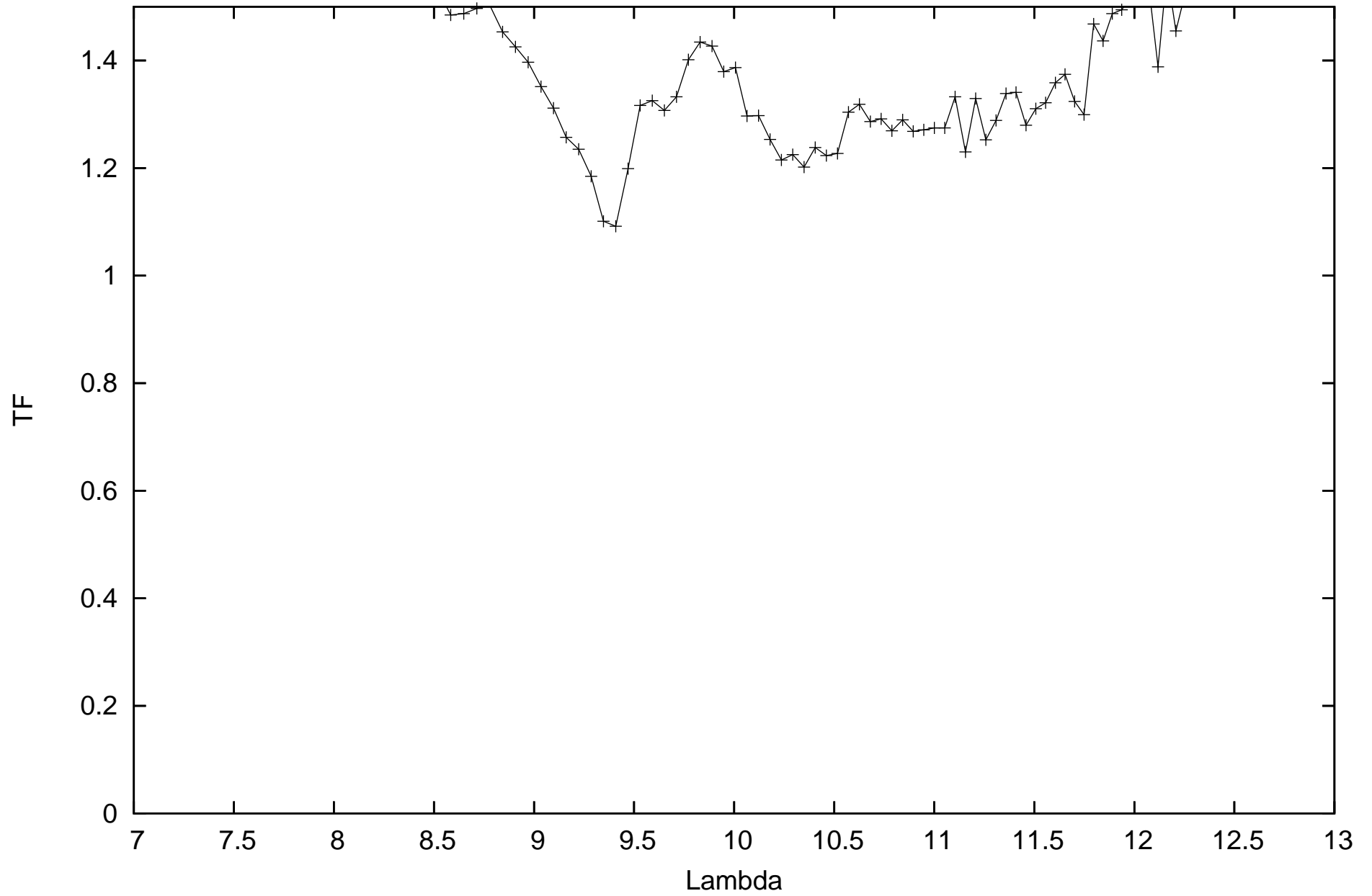
calHD048915_flux-1.39_diam6.09_r.MIDI.2009-01-17T06_20_20.137 SCIPHOT
