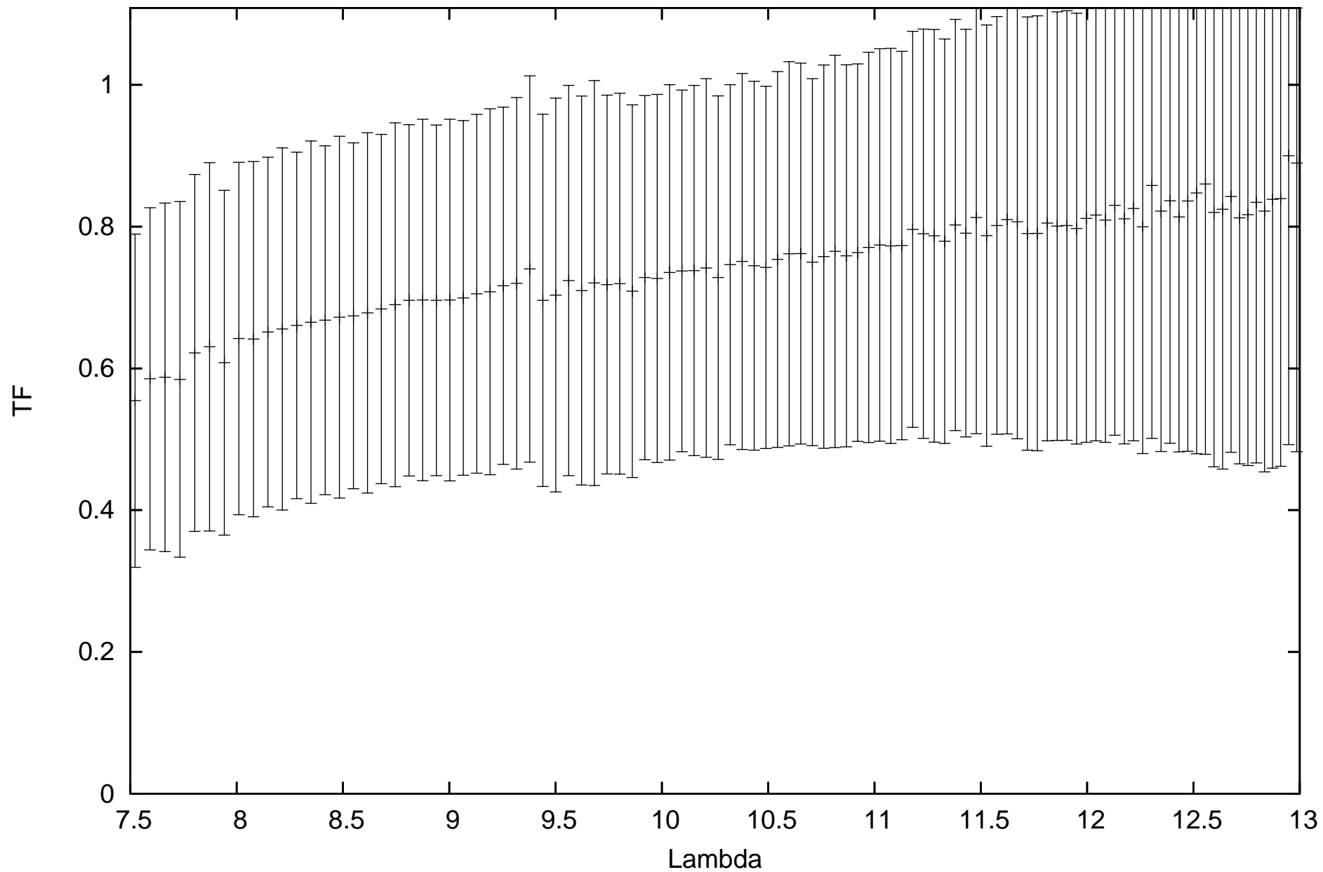
calHD048433_flux1.68_diam2.13_r.MIDI.2009-03-10T02_10_15.000_HIGHSENS
