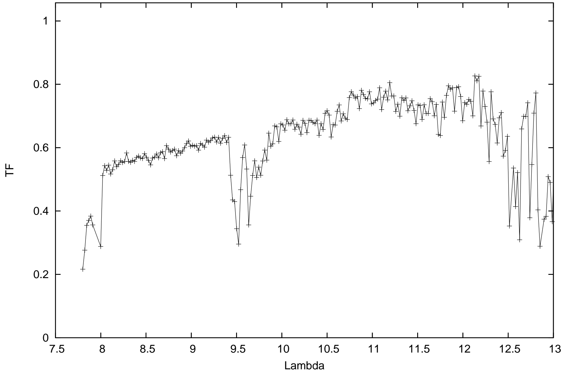
calHD048329_flux-0.02_diam4.56_r.MIDI.2010-01-17T05_48_31.000_E0G0
