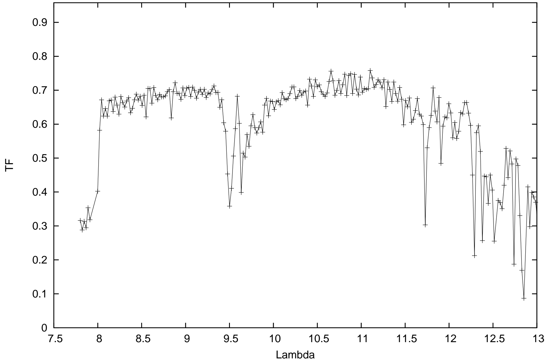
calHD048329_flux-0.02_diam4.56_r.MIDI.2009-01-21T04_05_03.000_HIGHSENS
