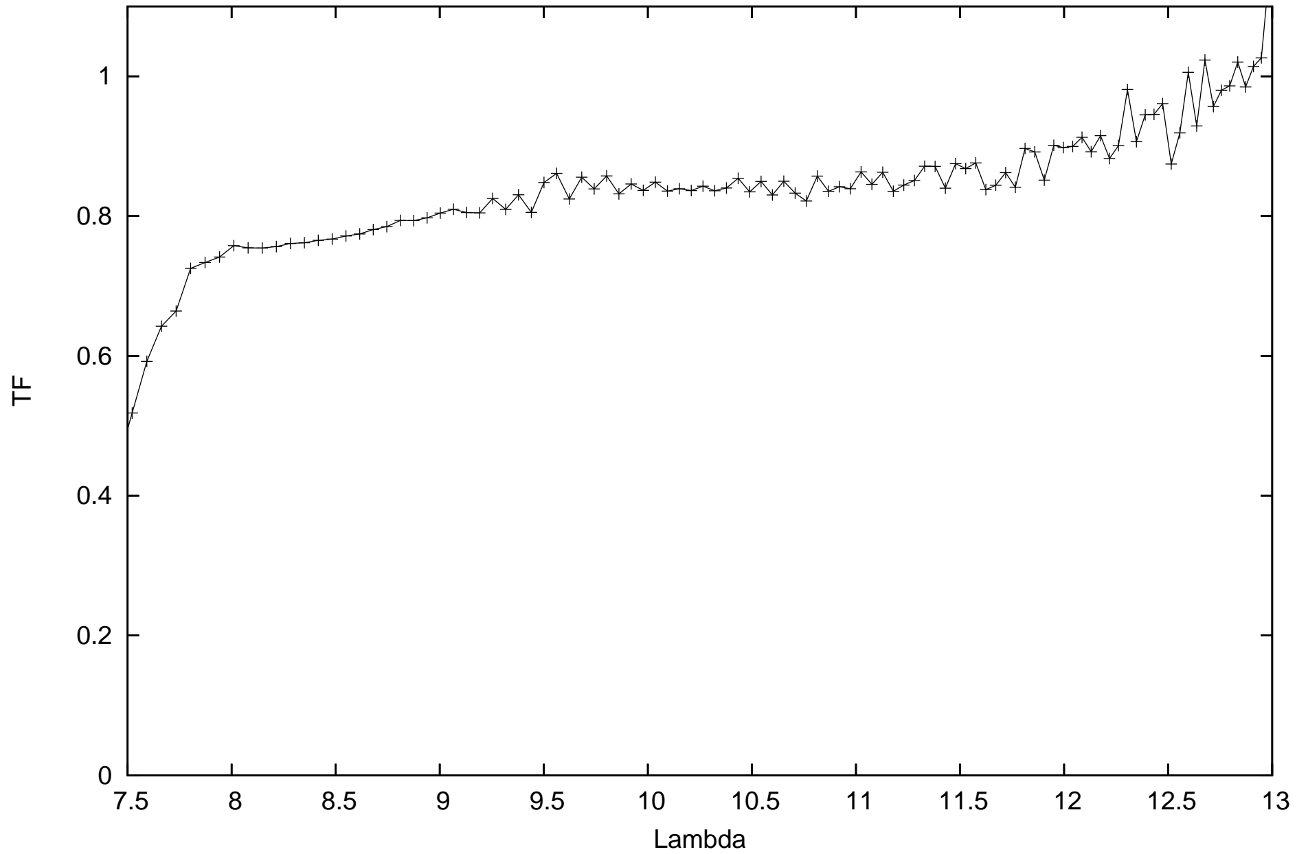
calHD045348_flux-1.47_diam6.87_r.MIDI.2009-02-23T02_52_00.000_HIGHSENS
