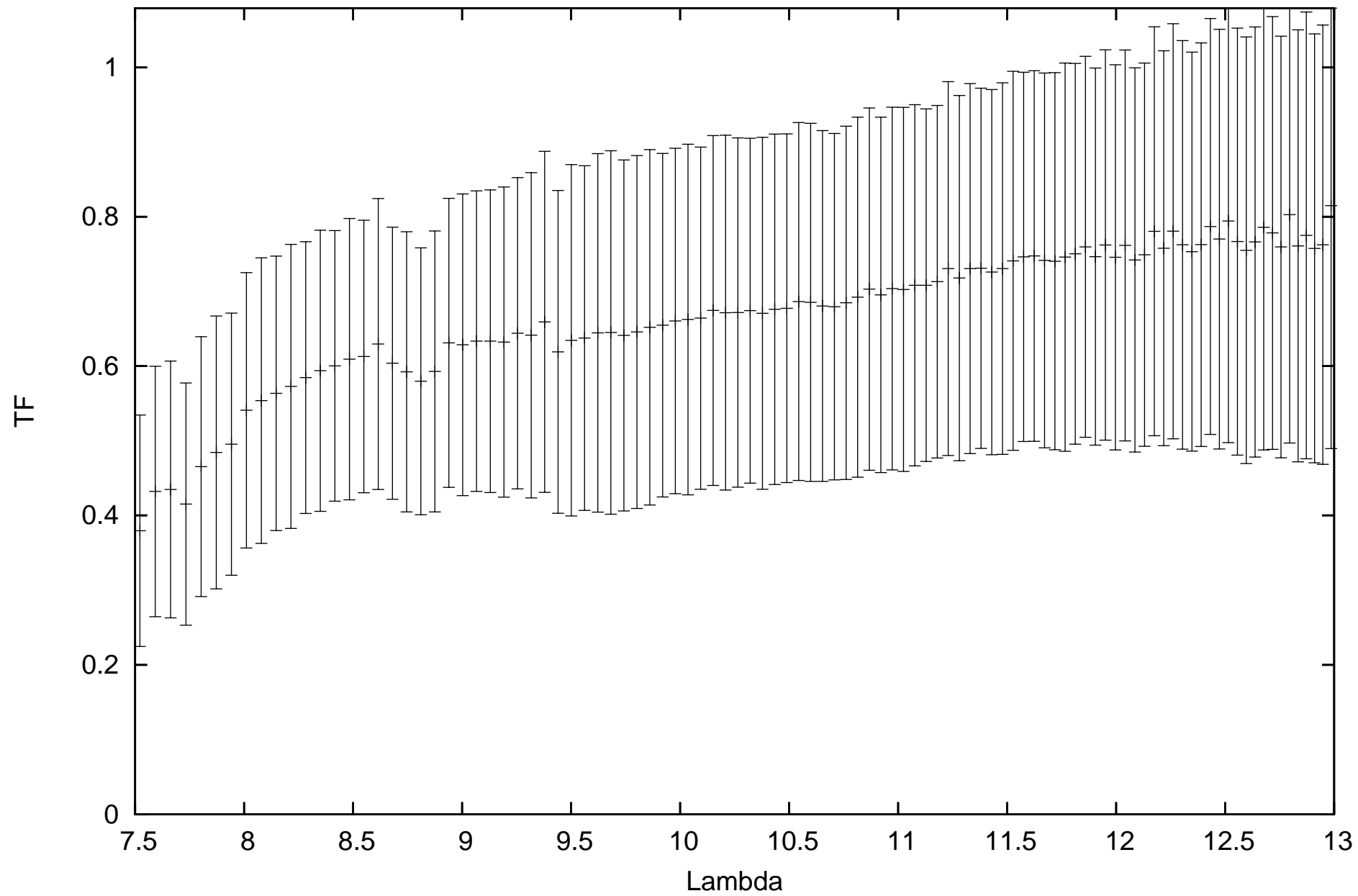
calHDO40808_flux1.31_diam2.43_r.MIDI.2009-05-09T23_07_47.000_U1U2
