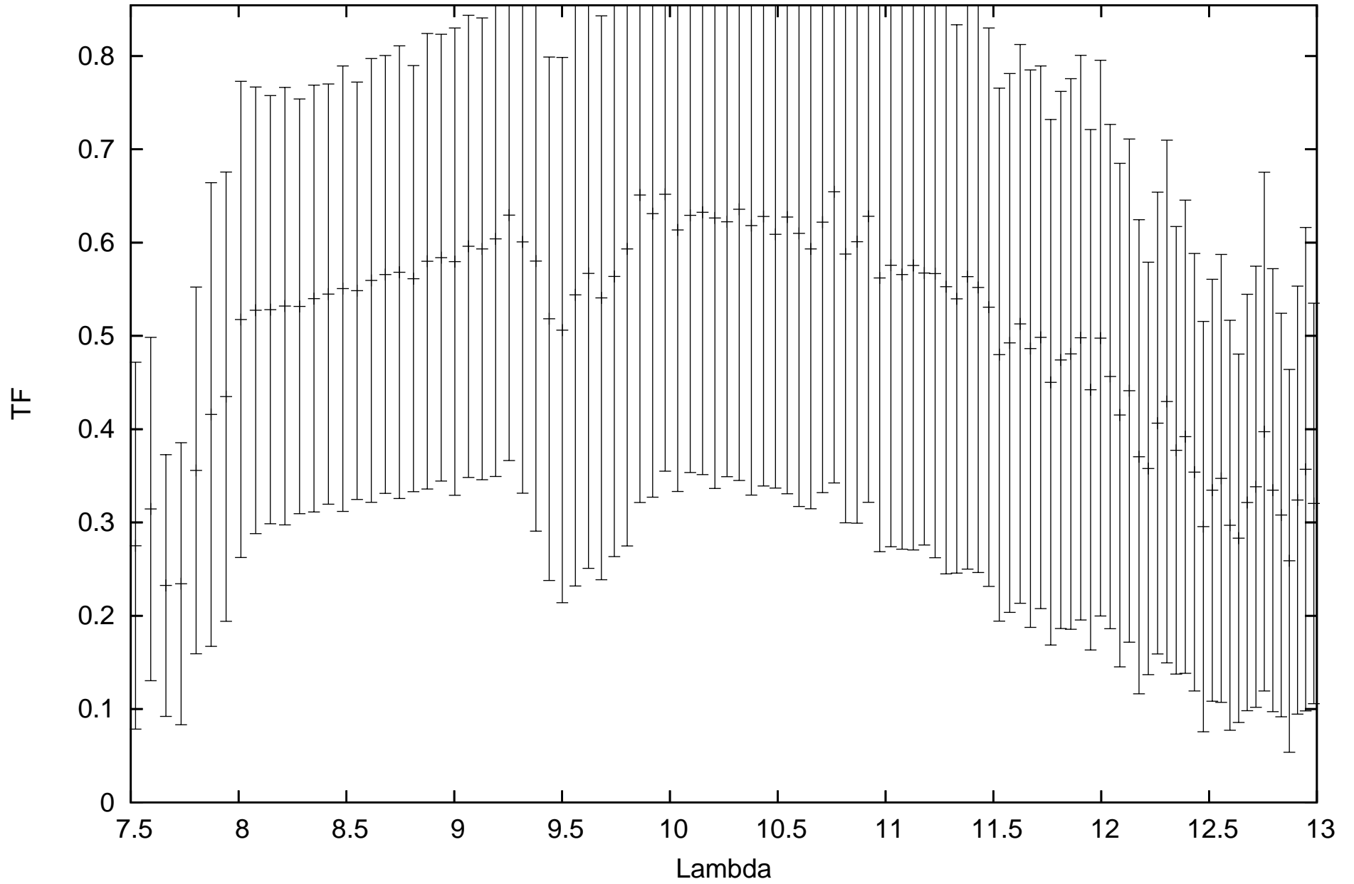
calHD039425_flux0.38_diam3.75_r.MIDI.2010-01-16T05_37_16.000_E0H0
