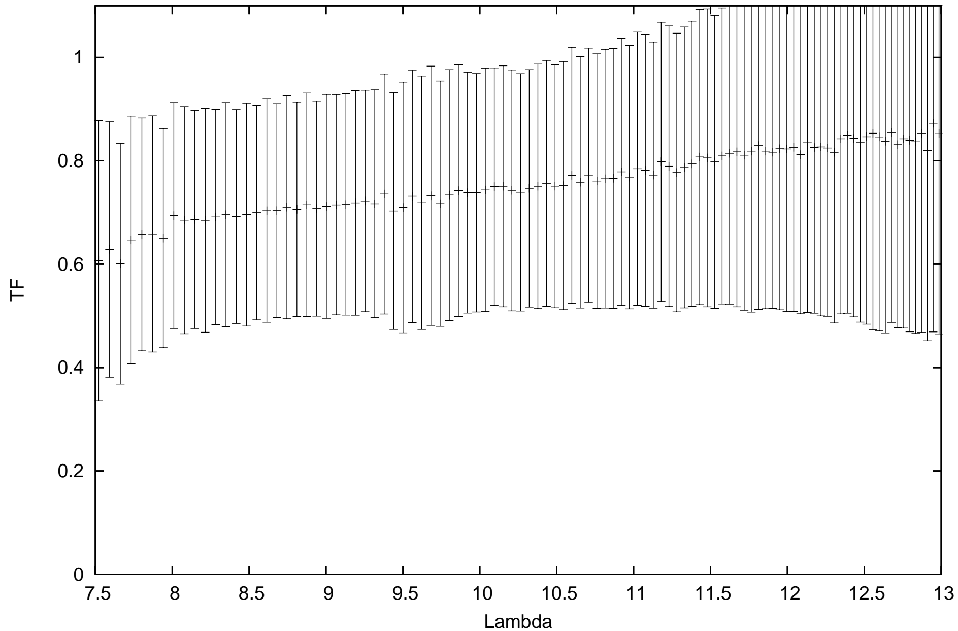
calHD039400_flux1.43_diam2.3_r.MIDI.2010-01-30T03_24_41.000_U2U4
