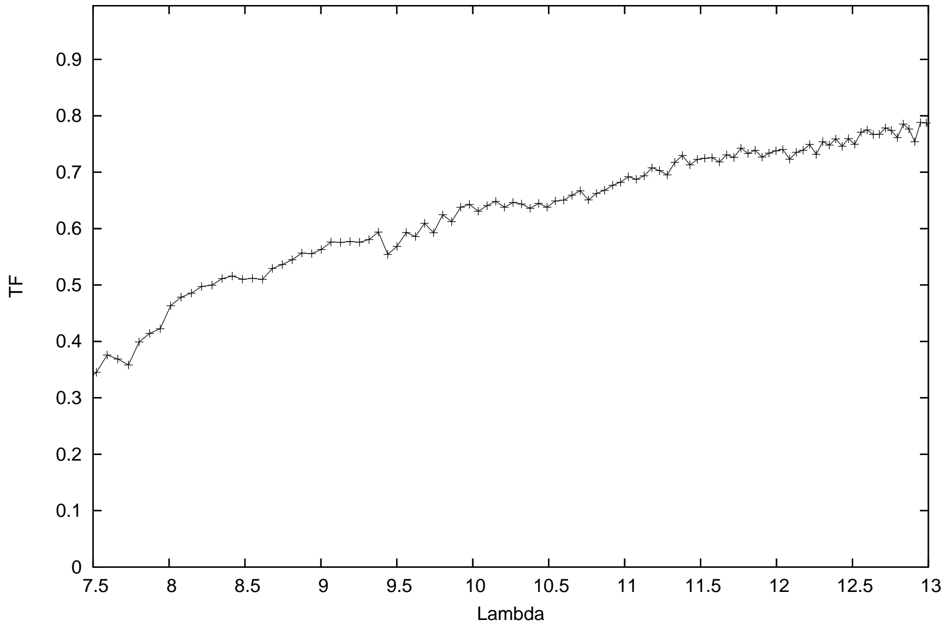
calHD036597_flux1.13_diam2.66_r.MIDI.2010-01-03T06_29_15.000_U3U4
