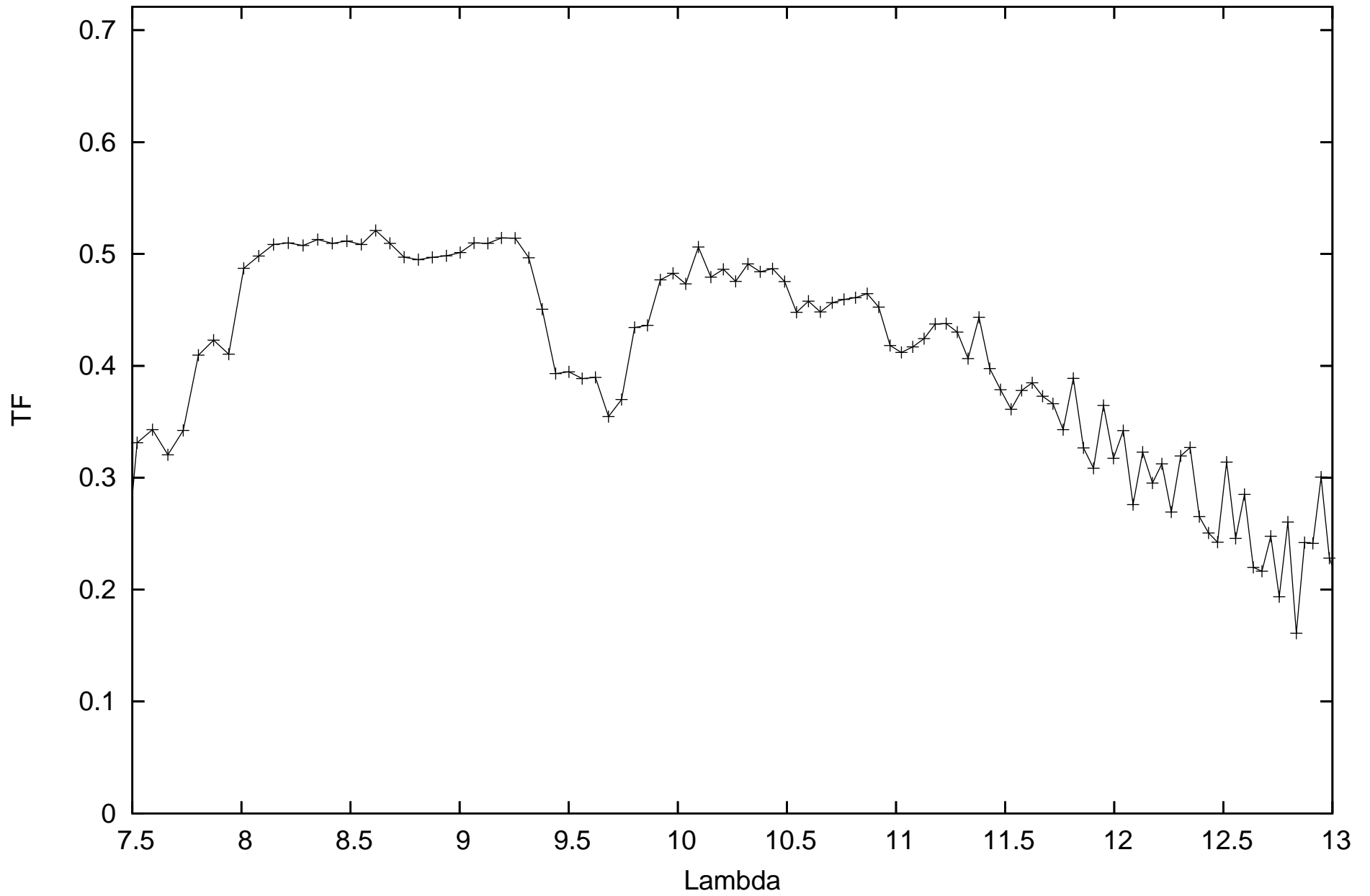
calHD036079_flux0.73_diam2.95_r.MIDI.2009-11-21T06_26_35.000_K0A0
