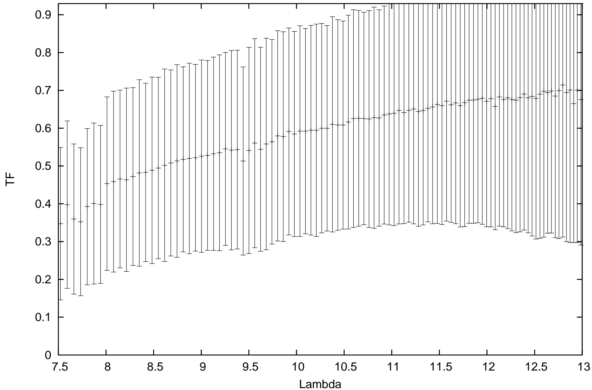
calHD033684_flux0.03_diam5.07_r.MIDI.2009-03-13T02_14_22.000_HIGHSENS
