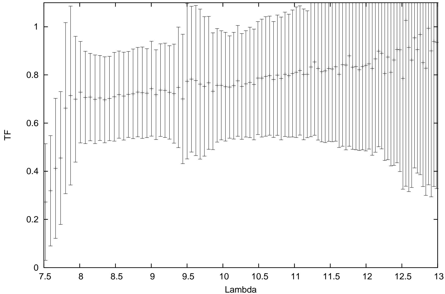
calHD031398_flux-0.85_diam7.1_r.MIDI.2009-02-17T00_44_24.000_HIGHSENS
