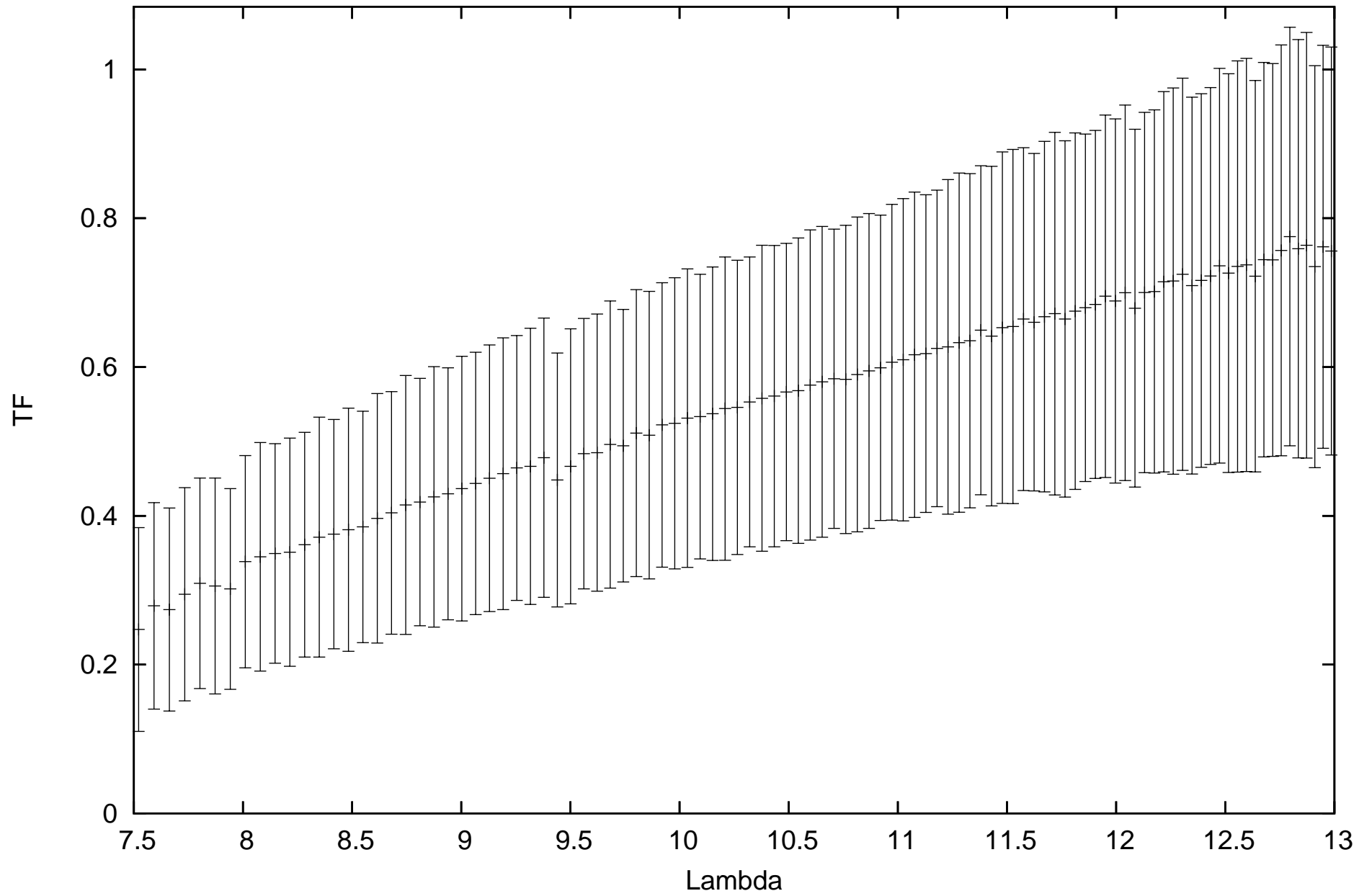
calHD029139_flux-3.11_diam20.4_r.MIDI.2010-01-13T02_27_10.000_G1D0
