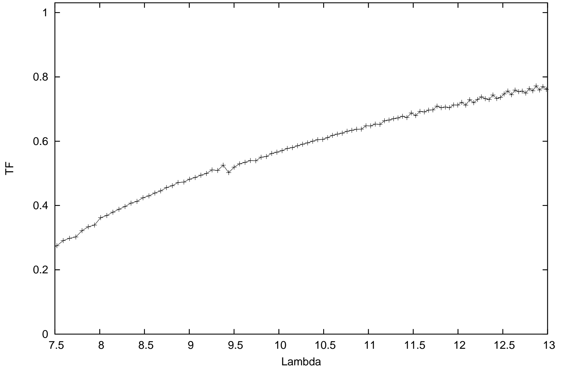
calHD029139_flux-3.11_diam20.4_r.MIDI.2010-01-11T02_46_48.000_H0D0
