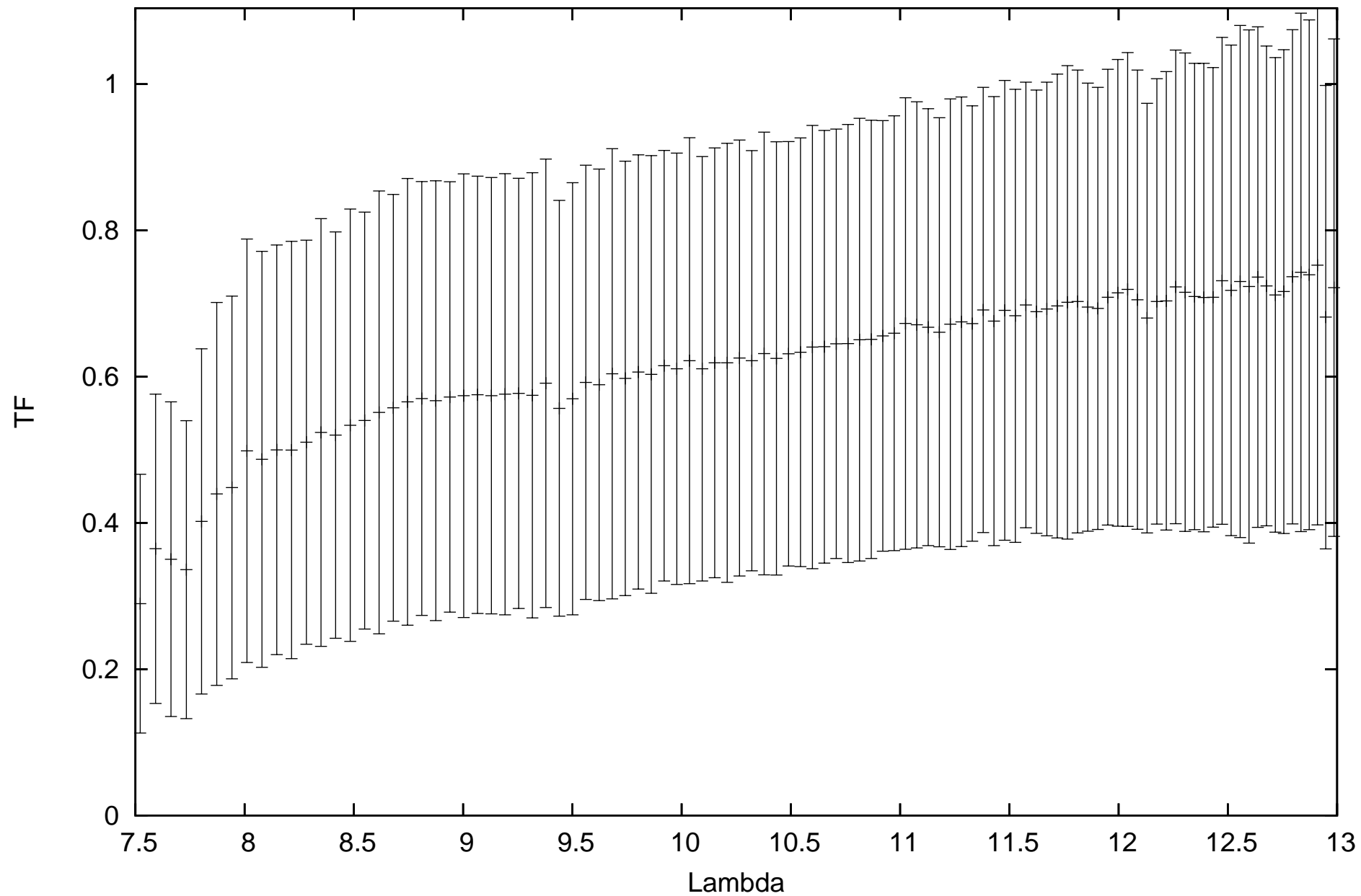
calHD026967_flux1.17_diam2.61_r.MIDI.2009-12-03T08_40_46.000_U2U4
