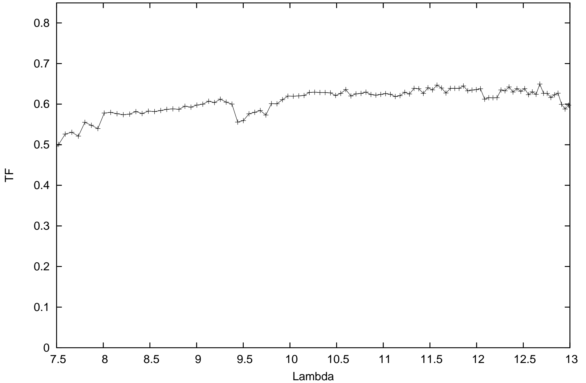
calHD020720_flux-1.53_diam10.14_r.MIDI.2010-01-11T04_04_21.000_H0D0
