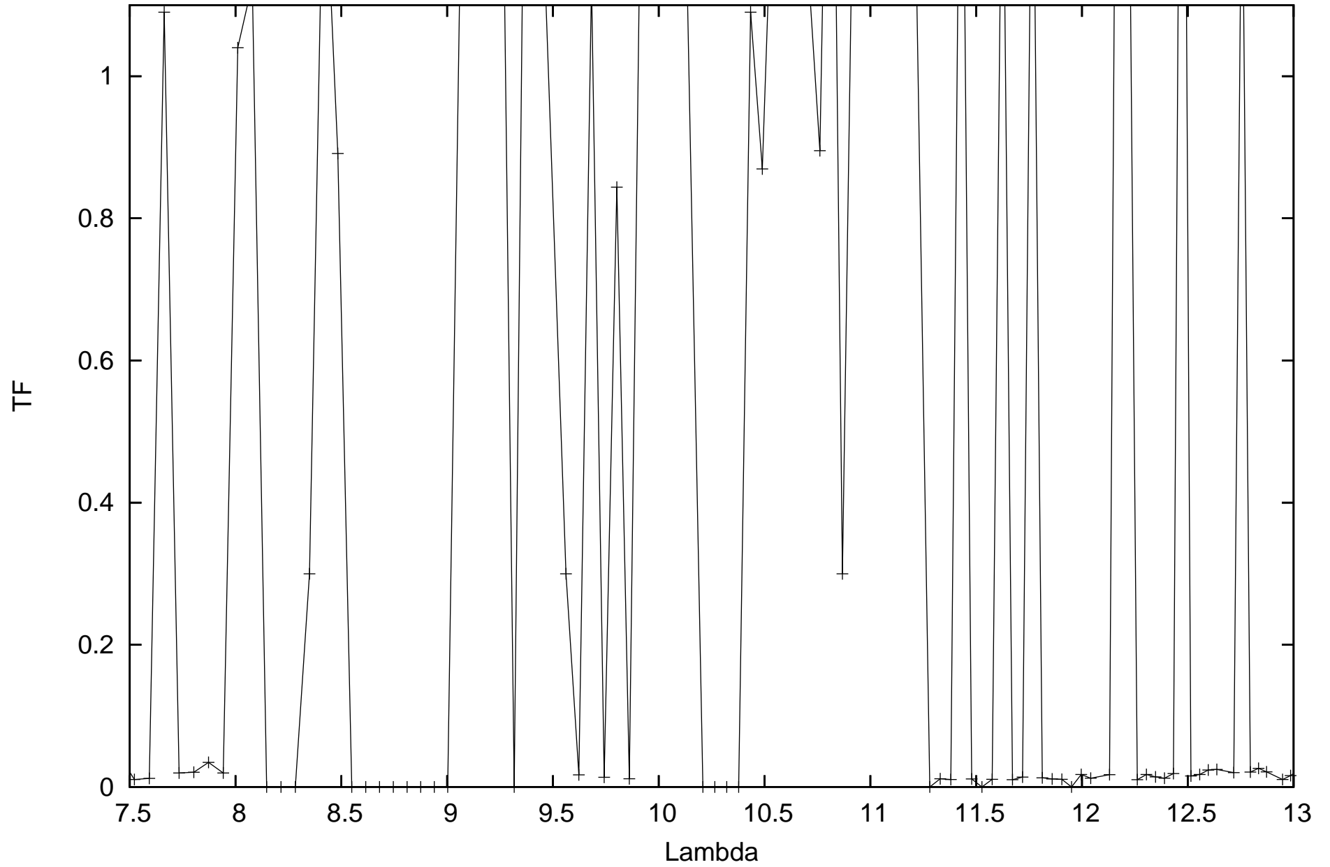
calHD018884_flux-1.93_diam12.27_r.MIDI.2009-01-04T01_31_15.000_HIGHSENS
