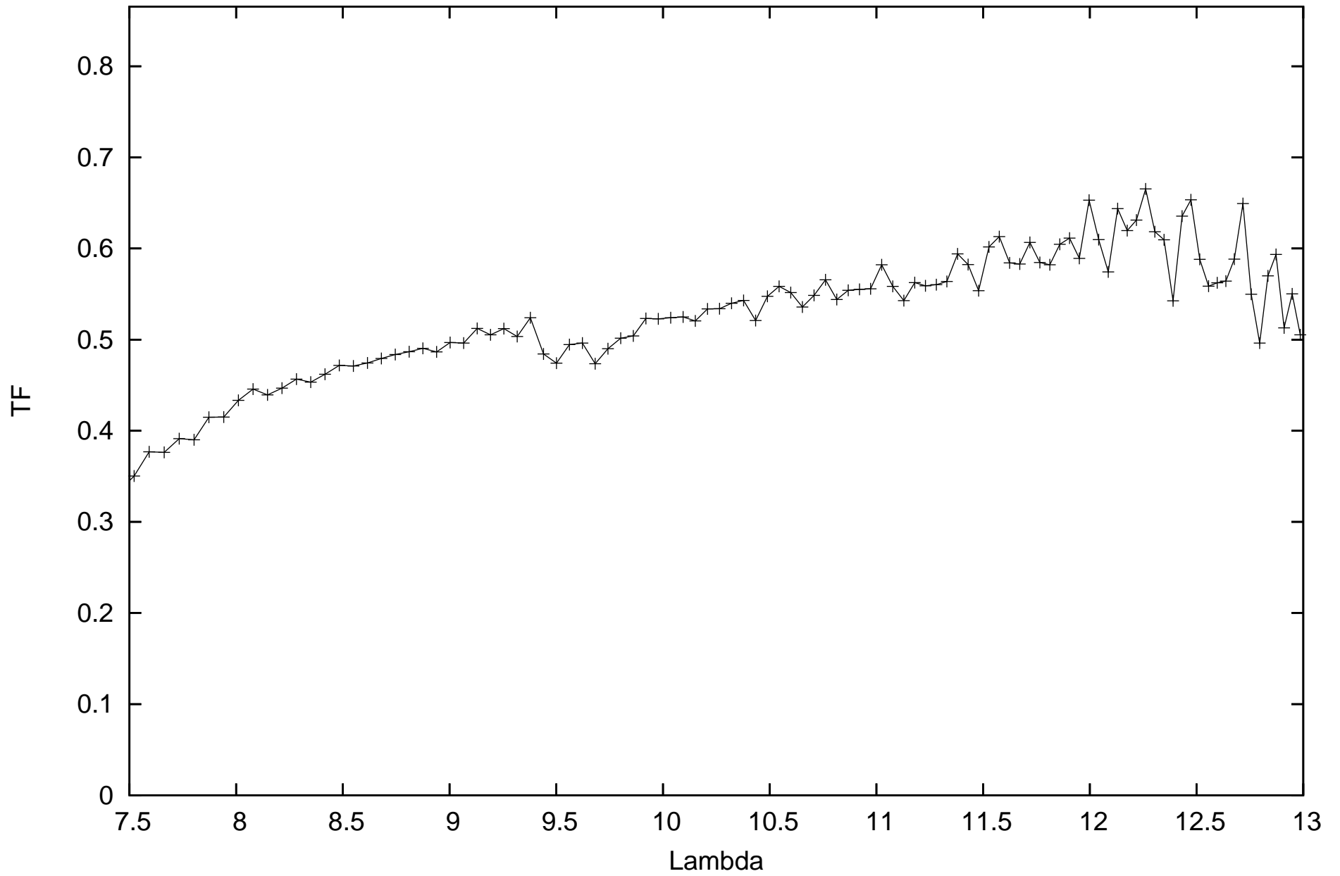
calHD004128_flux-0.44_diam5.23_r.MIDI.2009-09-21T05_55_44.000_HIGHSENS
