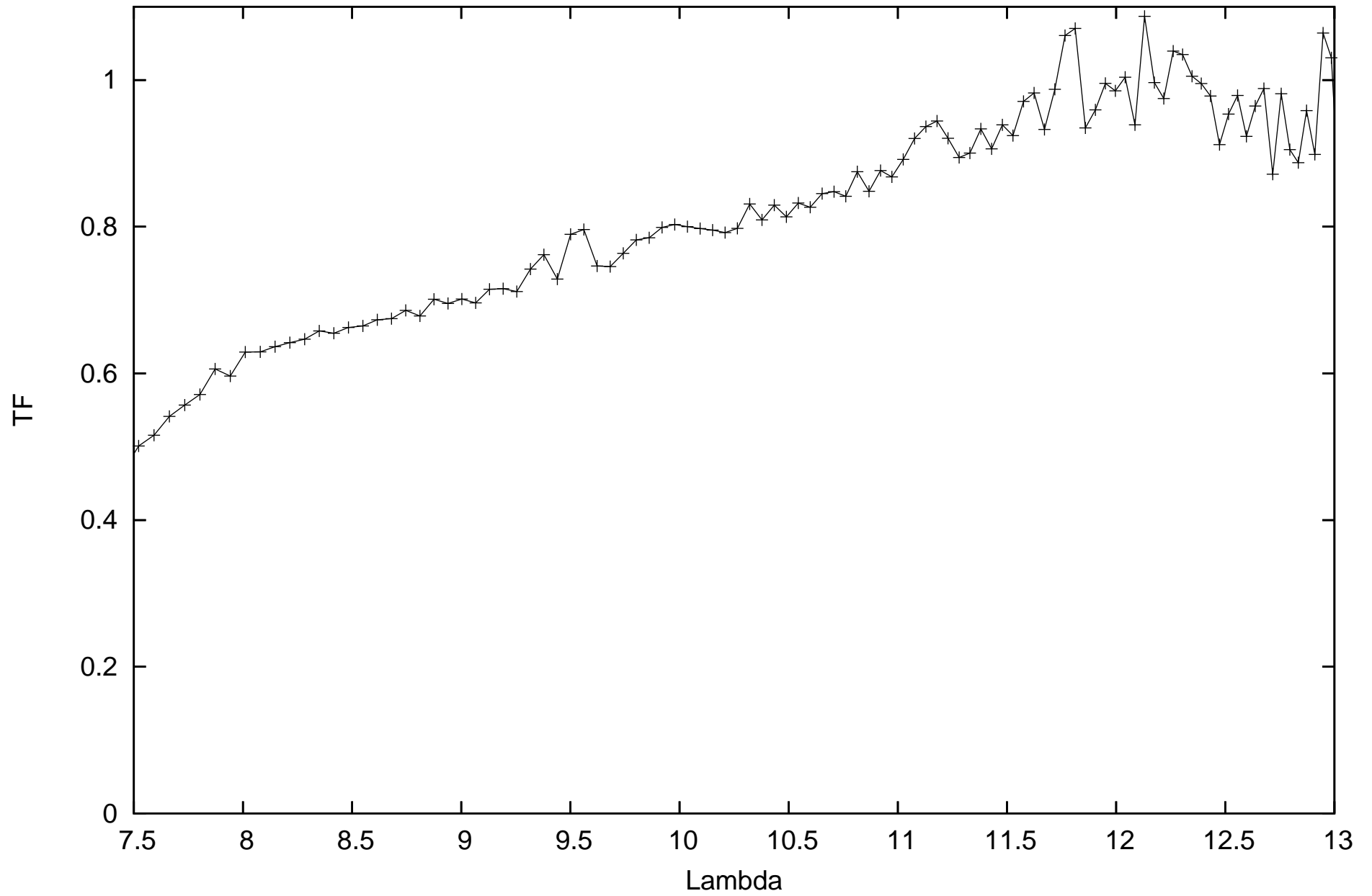
calHD004128_flux-0.44_diam5.23_r.MIDI.2009-09-20T06_22_33.000_HIGHSENS
