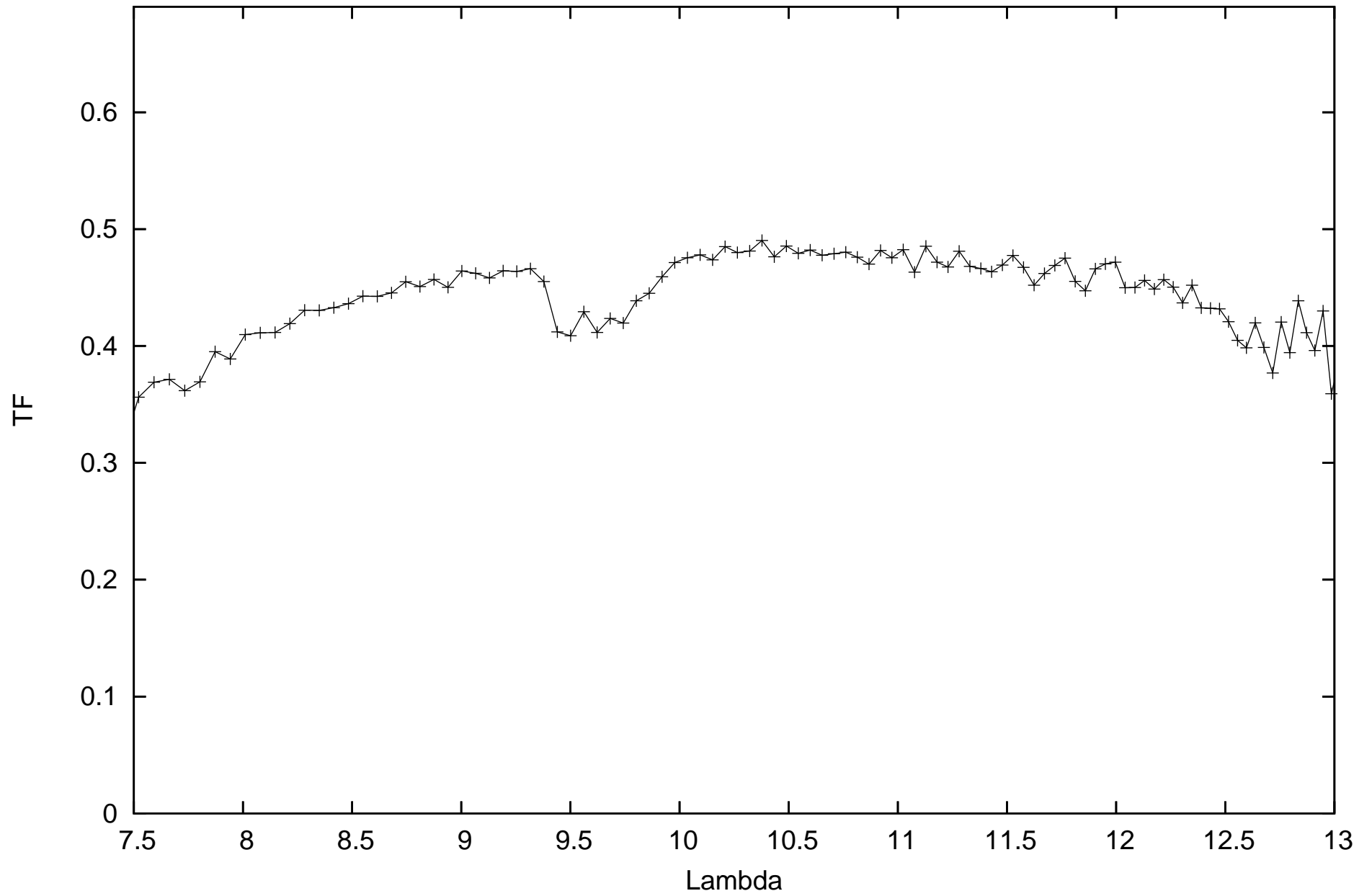
calHD004128_flux-0.44_diam5.23_r.MIDI.2009-09-06T09_26_13.000_HIGHSENS
