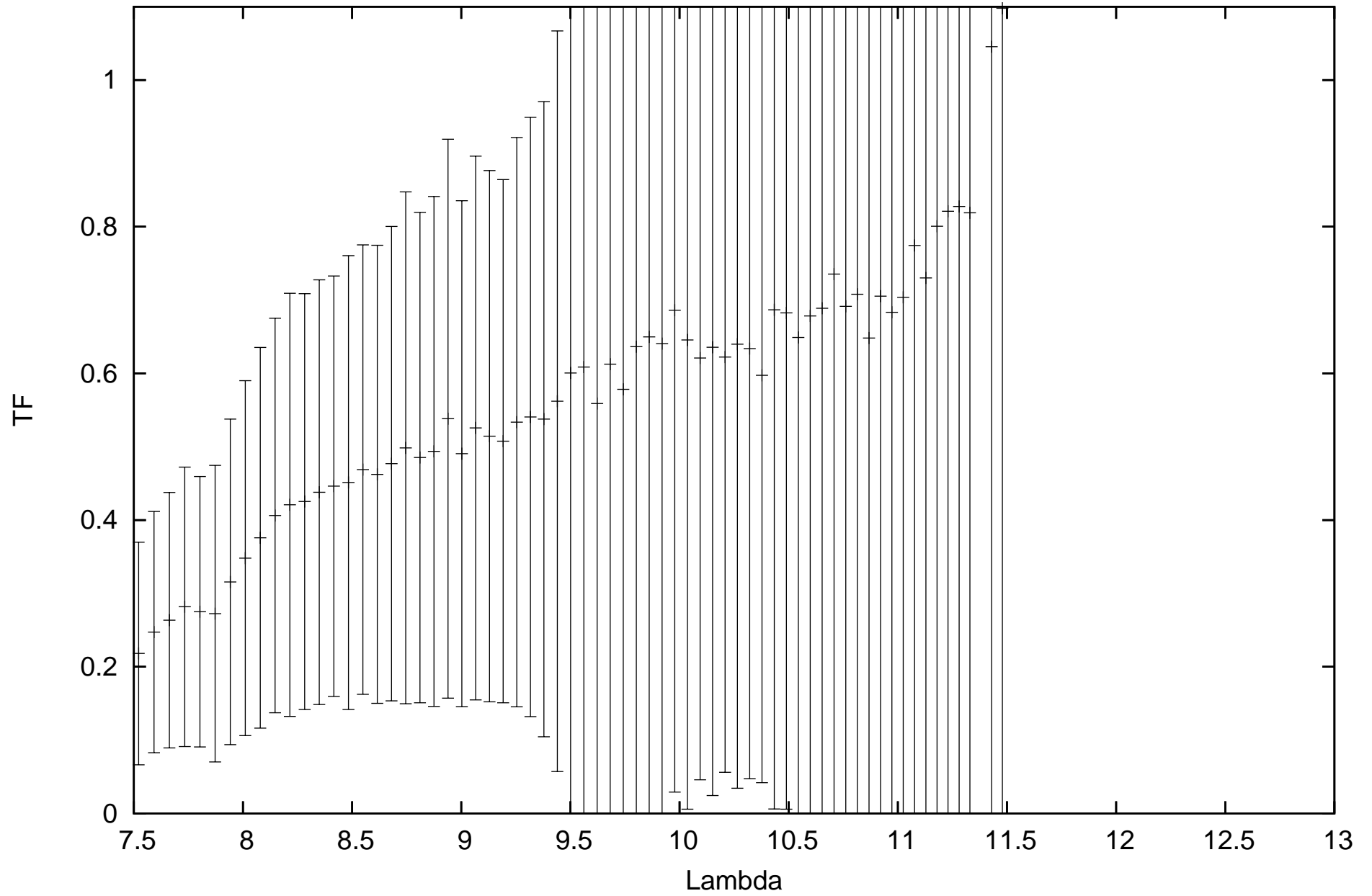
calHD001038_flux-0.08_diam5.17_r.MIDI.2008-09-27T05_43_54.000_HIGHSENS
