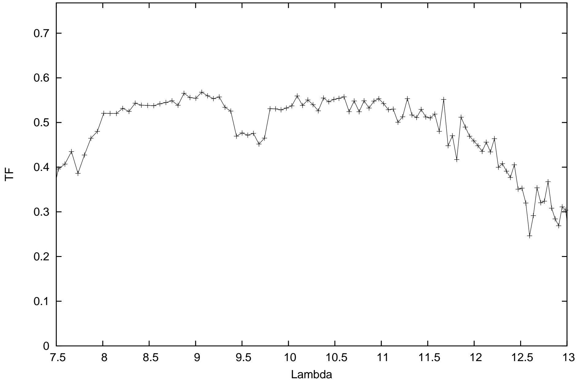
calHD001014_flux0.24_diam4.61_r.MIDI.2009-11-18T01_51_18.000_K0A0
