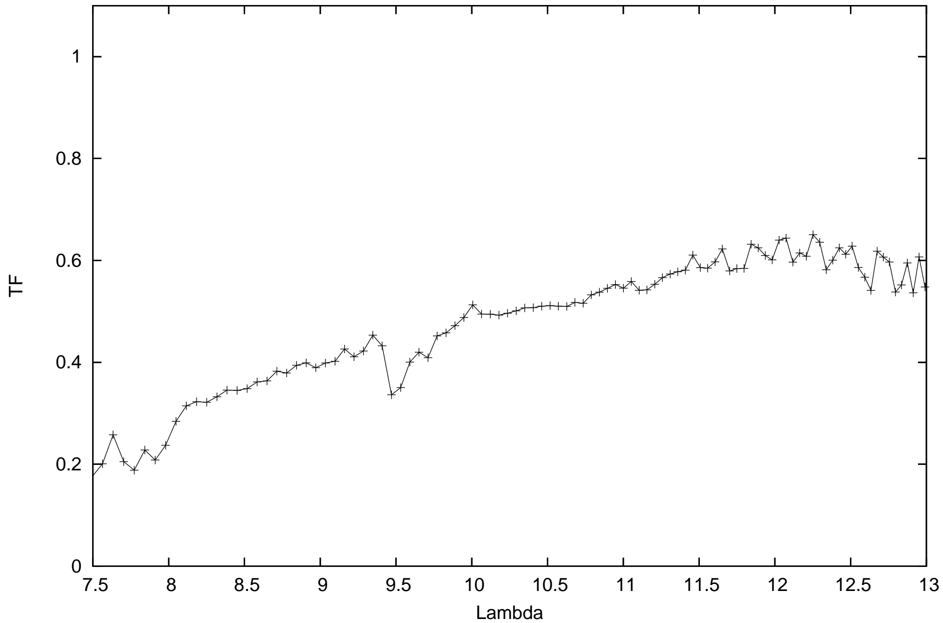
calHD216131_flux1.28_diam2.46_r.MIDI.2009-12-04T00_36_11.686_U1U2
