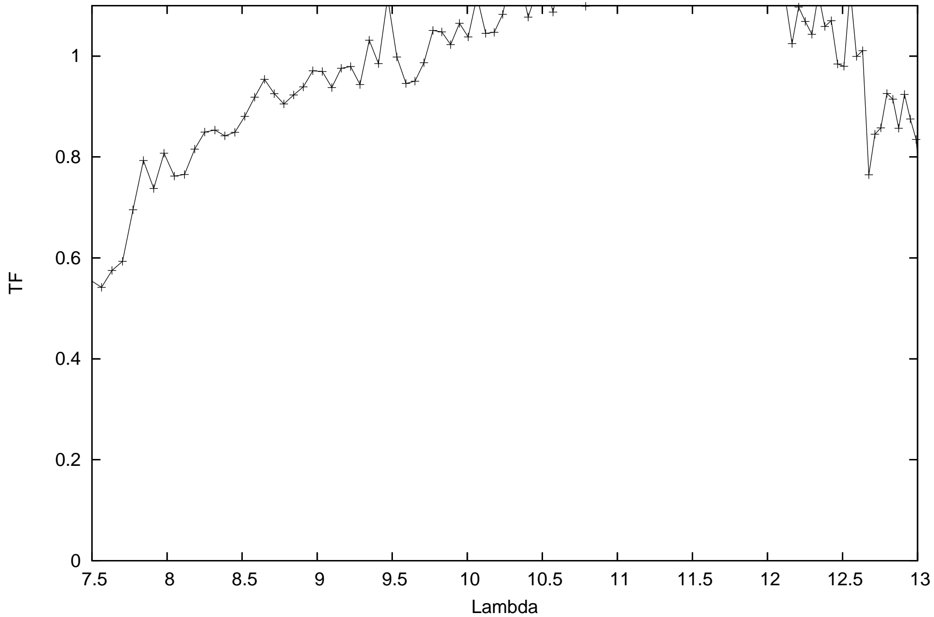
calHD206778_flux-1.04_diam7.59_r.MIDI.2009-11-15T01_13_42.686_E0G0
