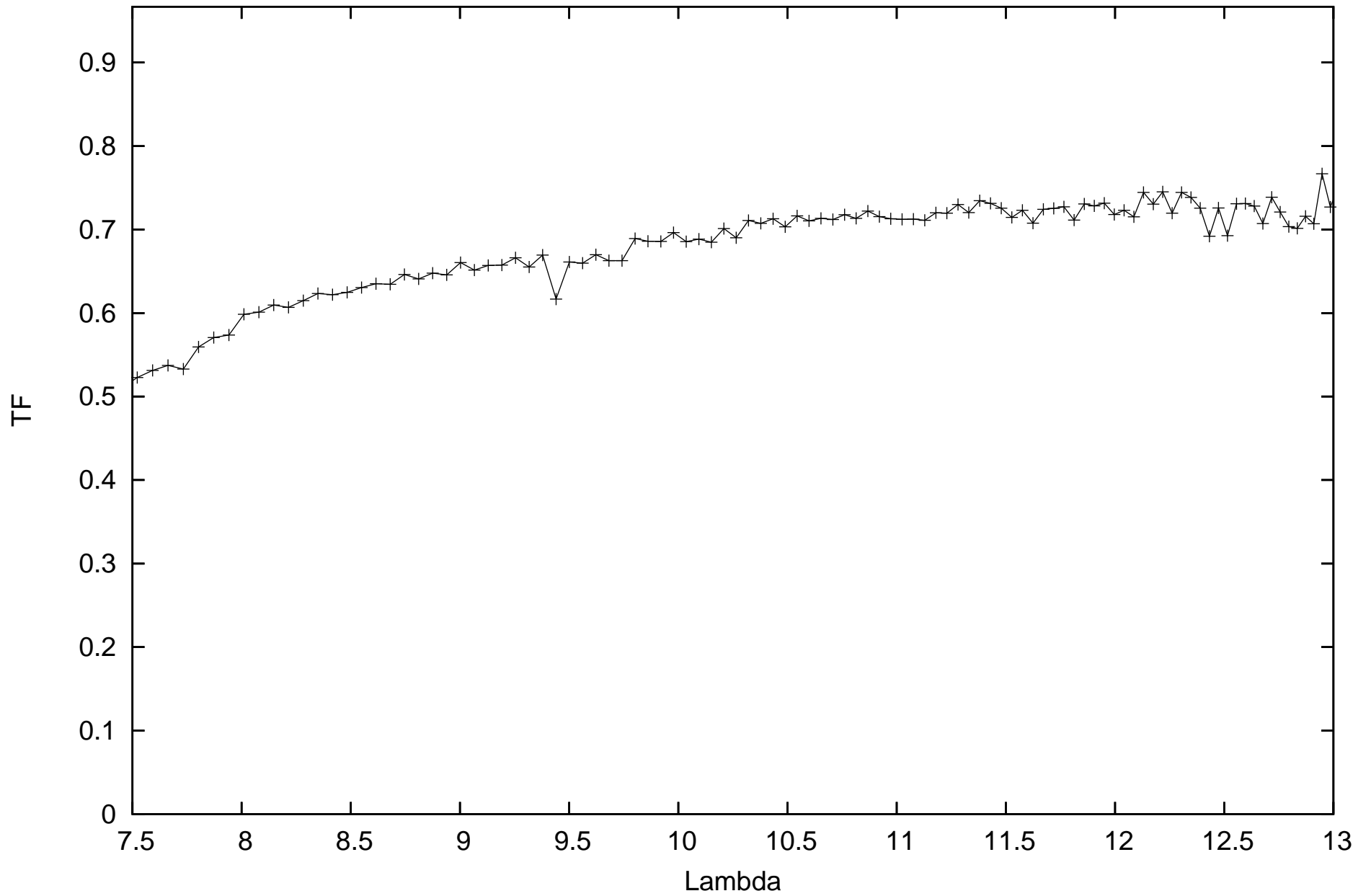
calHD206778_flux-1.04_diam7.59_r.MIDI.2009-11-15T00_13_54.000_E0G0
