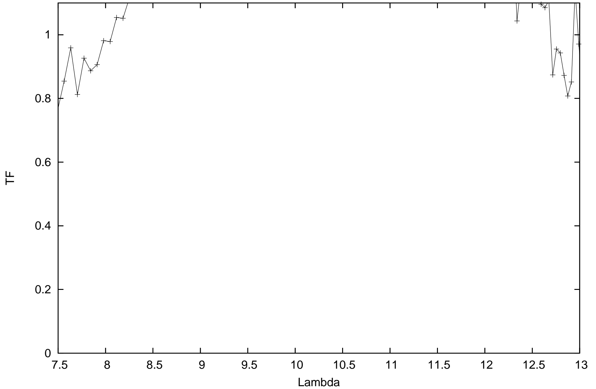
calHD224935_flux-0.85_diam7.24_r.MIDI.2009-10-31T04_35_23.686_H0G0
