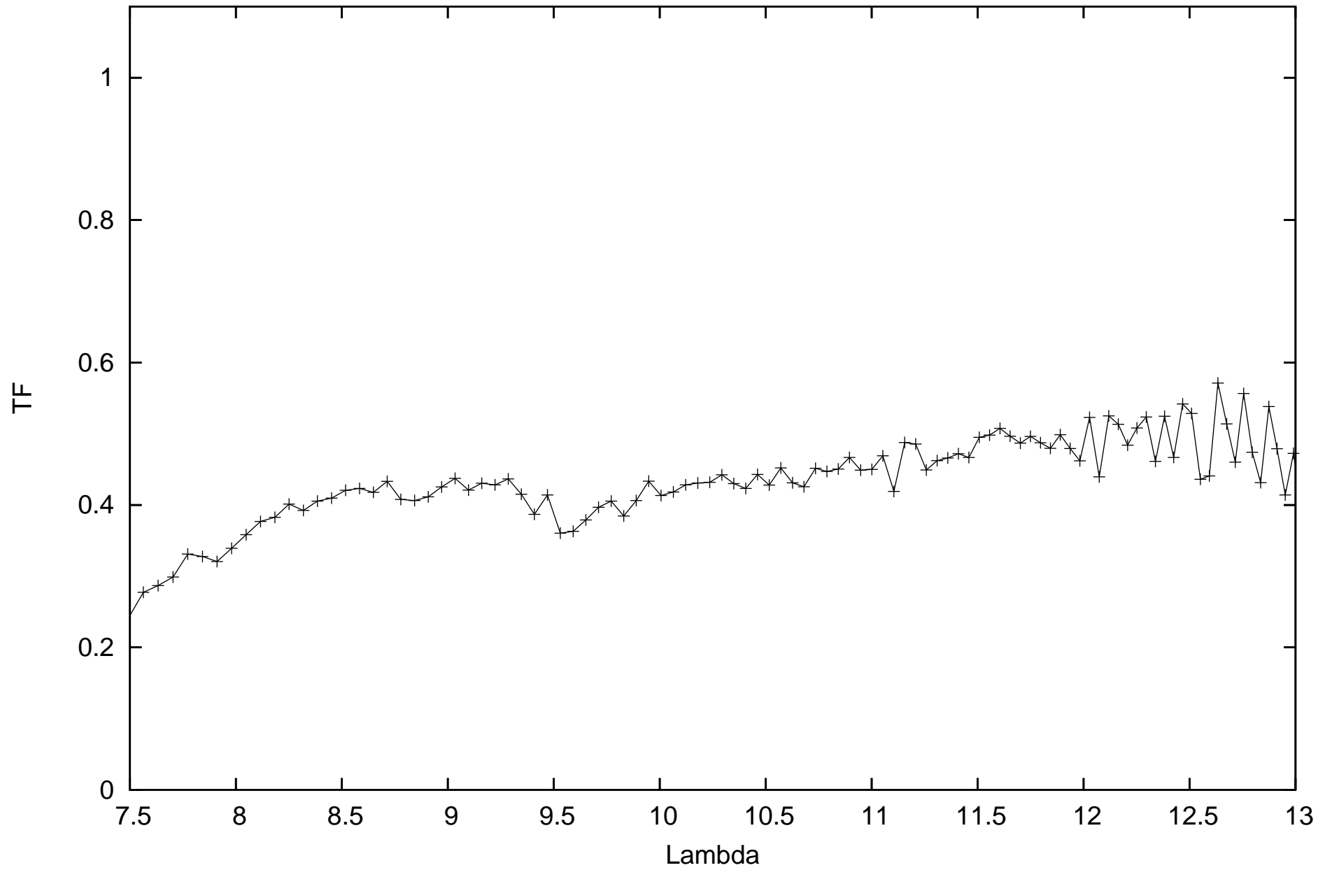
calHD224935_flux-0.85_diam7.24_r.MIDI.2009-10-02T04_15_51.686_H0G0
