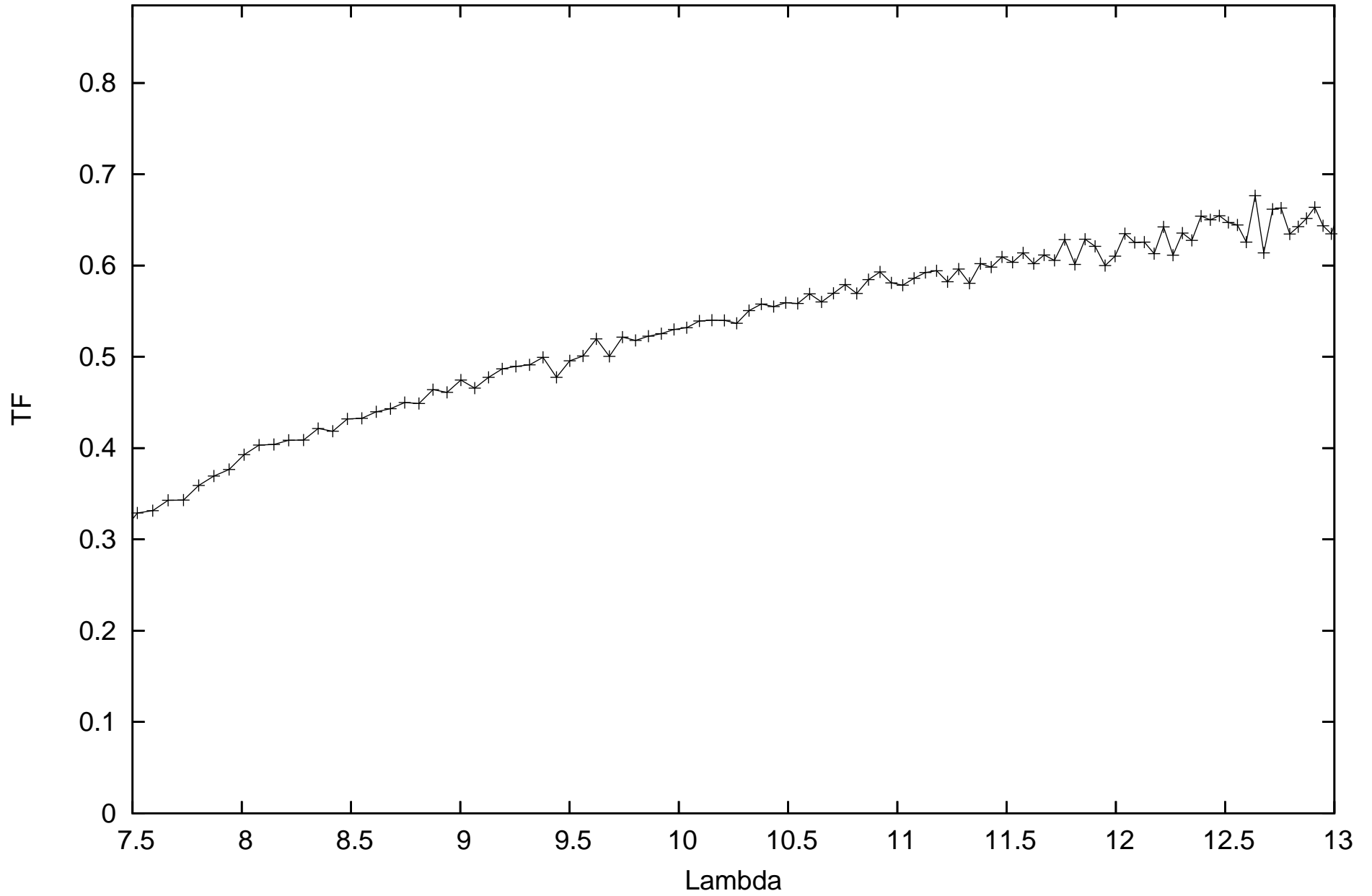
calHD020720_flux-1.53_diam10.14_r.MIDI.2009-09-07T09_27_37.000_HIGHSENS
