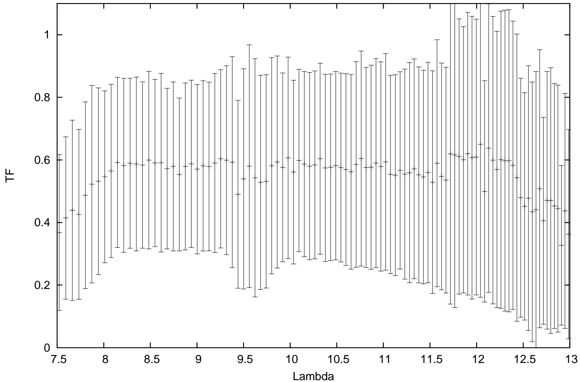
calHD169916_flux0.26_diam3.99_r.MIDI.2009-08-18T04_30_40.000_HIGHSENS
