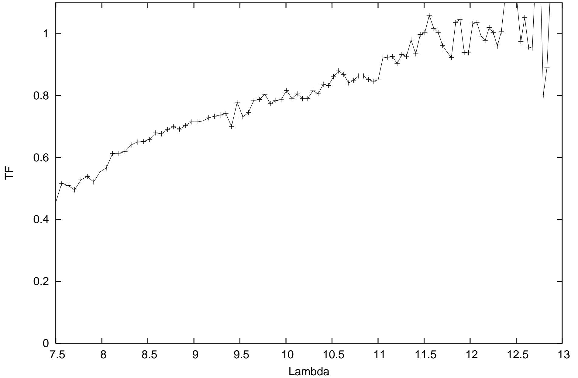
calHD224935_flux-0.85_diam7.24_r.MIDI.2009-08-14T09_07_14.686 SCIPHOT
