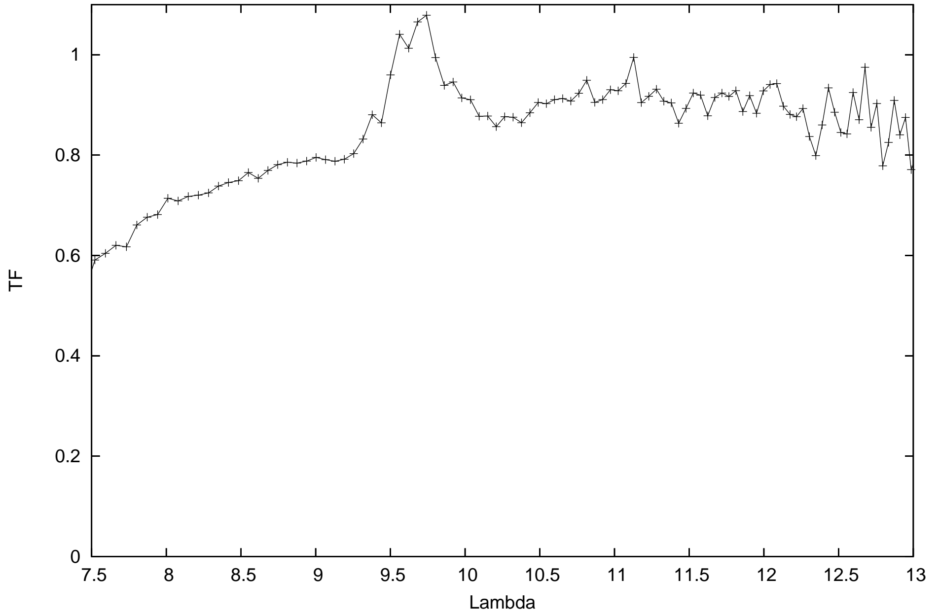
calHD189319_flux-0.43_diam5.93_r.MIDI.2009-08-14T04_11_00.000_HIGHSENS
