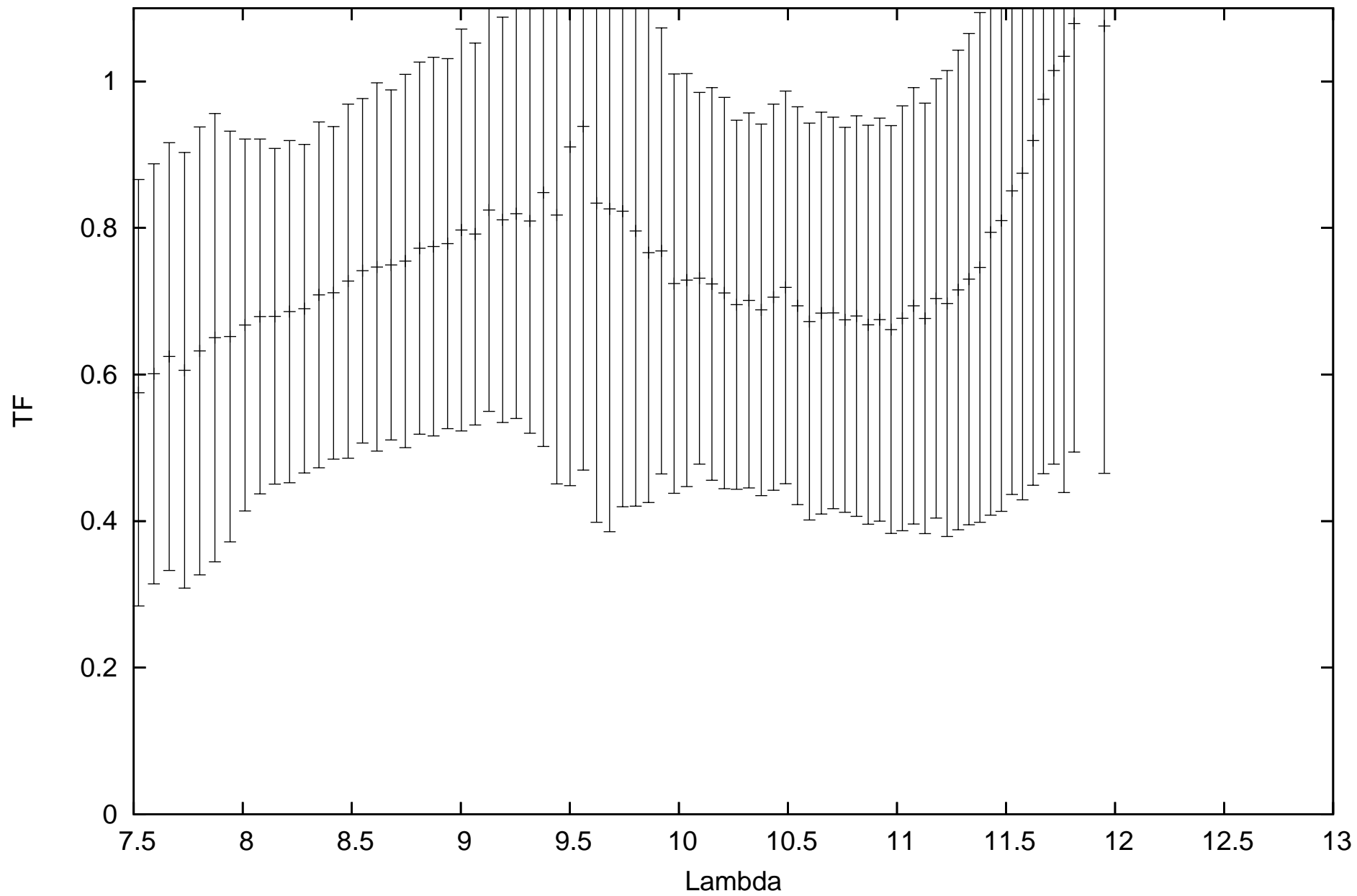
calHD161096_flux0.03_diam4.37_r.MIDI.2009-08-14T02_21_05.000_HIGHSENS
