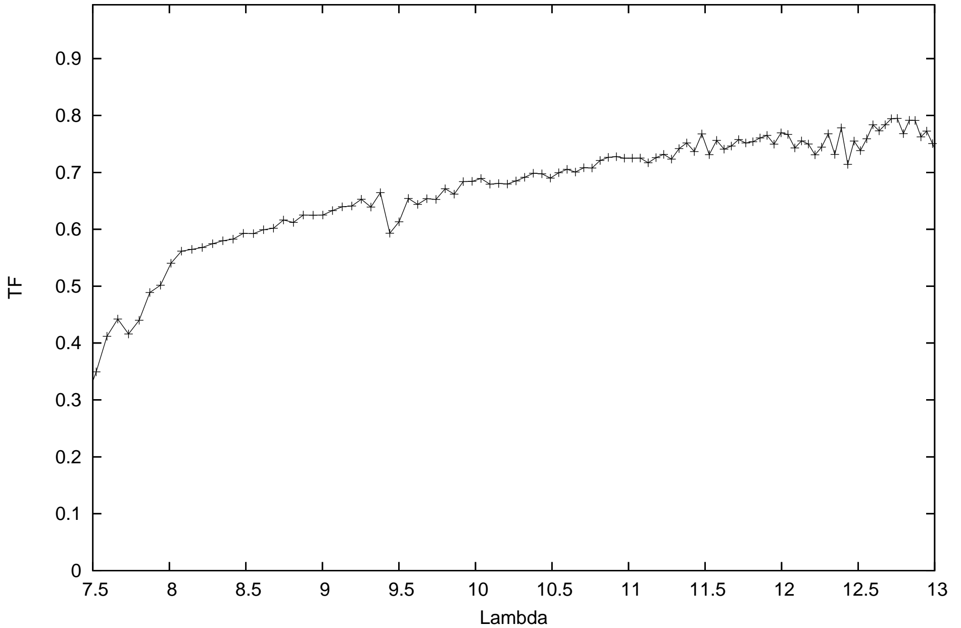
calHD171759_flux1.17_diam2.68_r.MIDI.2009-08-04T06_00_28.000_HIGHSENS
