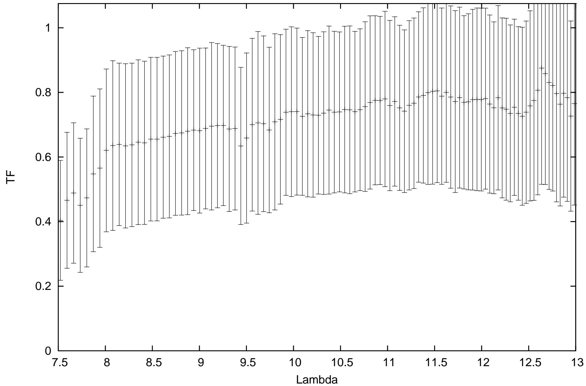
calHD156277_flux1.83_diam2._r.MIDI.2009-08-04T05_04_54.000_HIGHSENS
