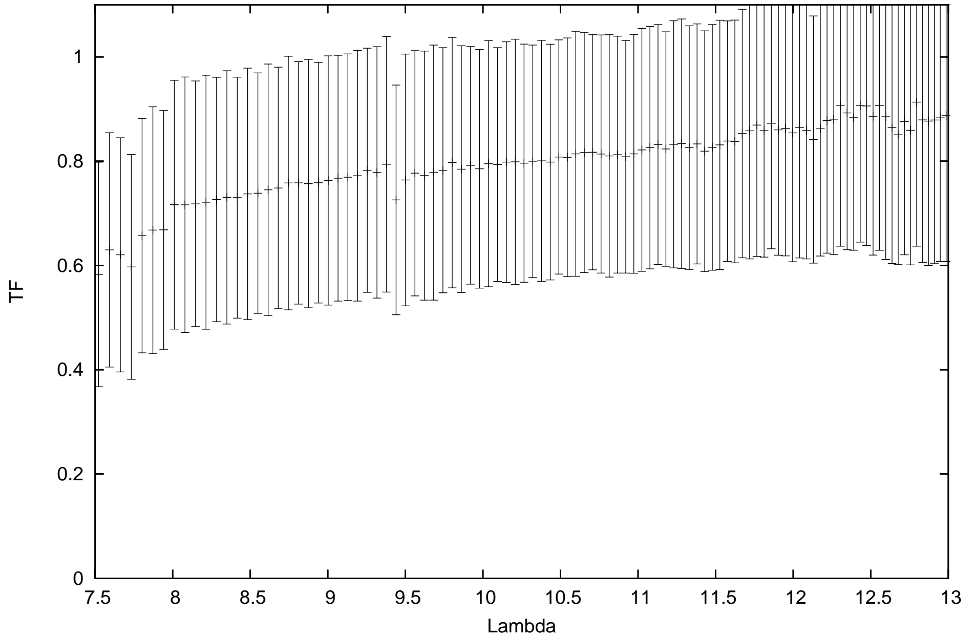
calHD171759_flux1.17_diam2.68_r.MIDI.2009-08-03T06_03_35.000_HIGHSENS
