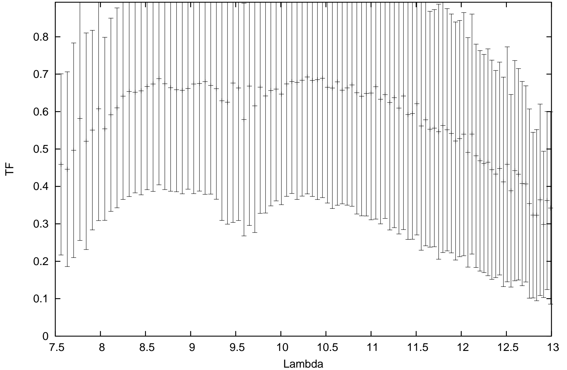
calHD081797_flux-1.49_diam9.14_r.MIDI.2009-05-20T01_01_50.809 SCIPHOT
