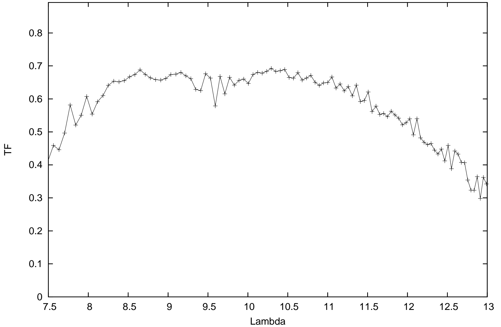
calHD081797_flux-1.49_diam9.14_r.MIDI.2009-05-20T01_01_50.809 SCIPHOT
