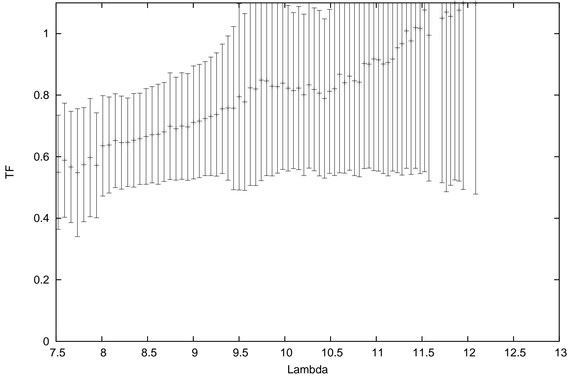
calHD168454_flux-0.48_diam5.87_r.MIDI.2009-05-03T09_57_25.000_HIGHSENS
