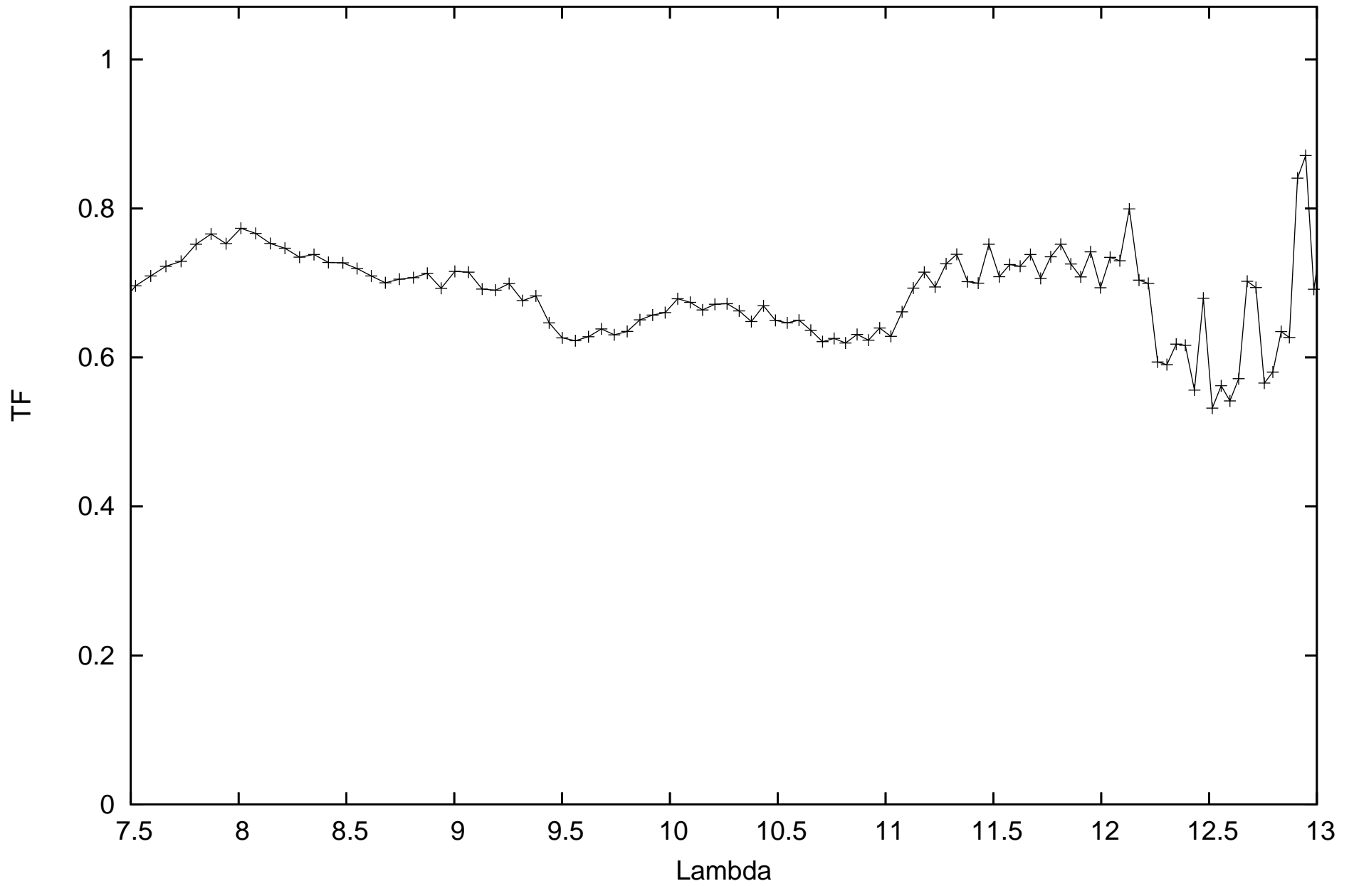
calHD093813_flux0.14_diam4.43_r.MIDI.2009-04-21T04_05_28.000_HIGHSENS
