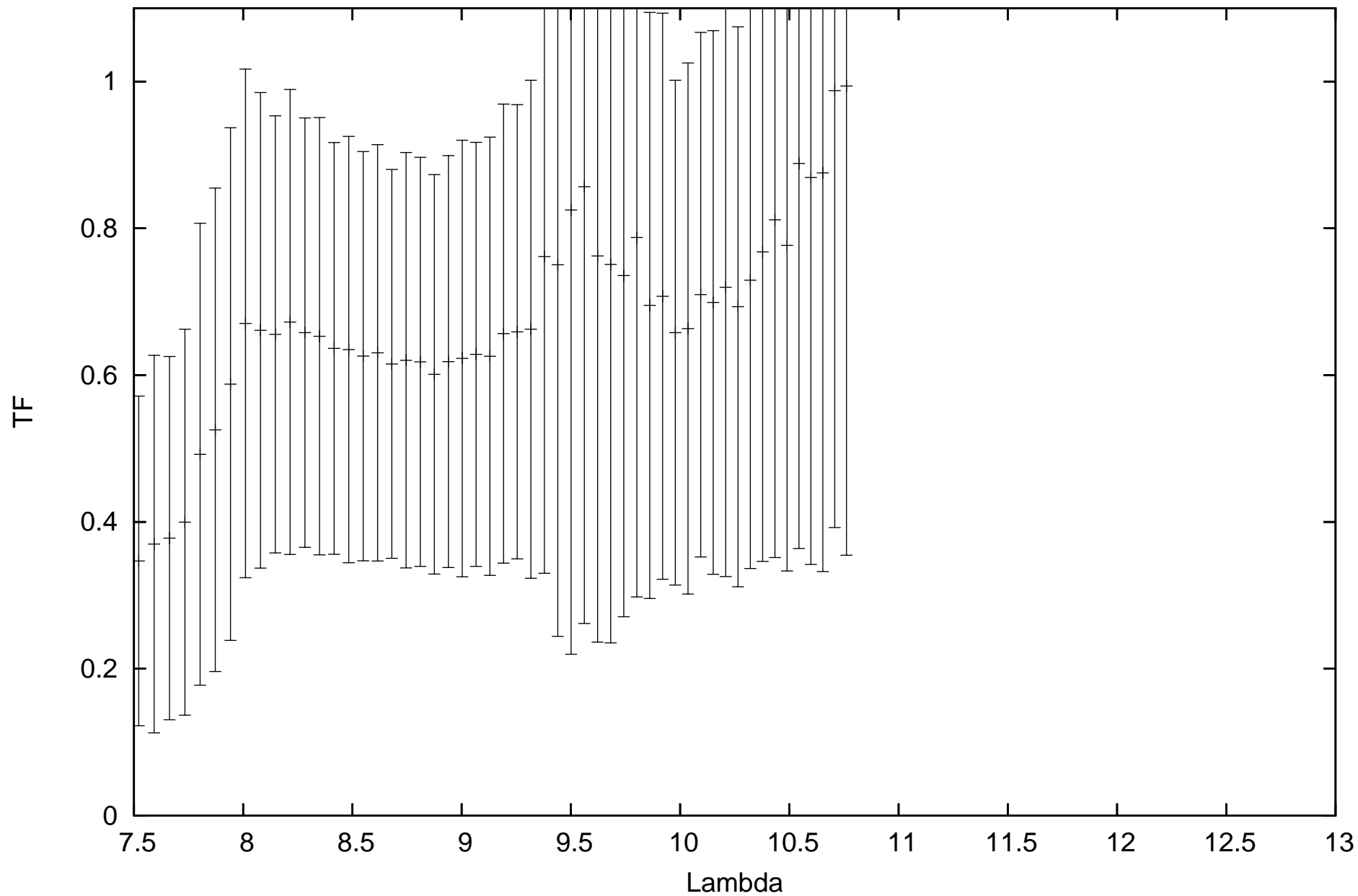
calHD092036_flux0.5_diam4.05_r.MIDI.2009-04-19T03_07_32.000_HIGHSENS
