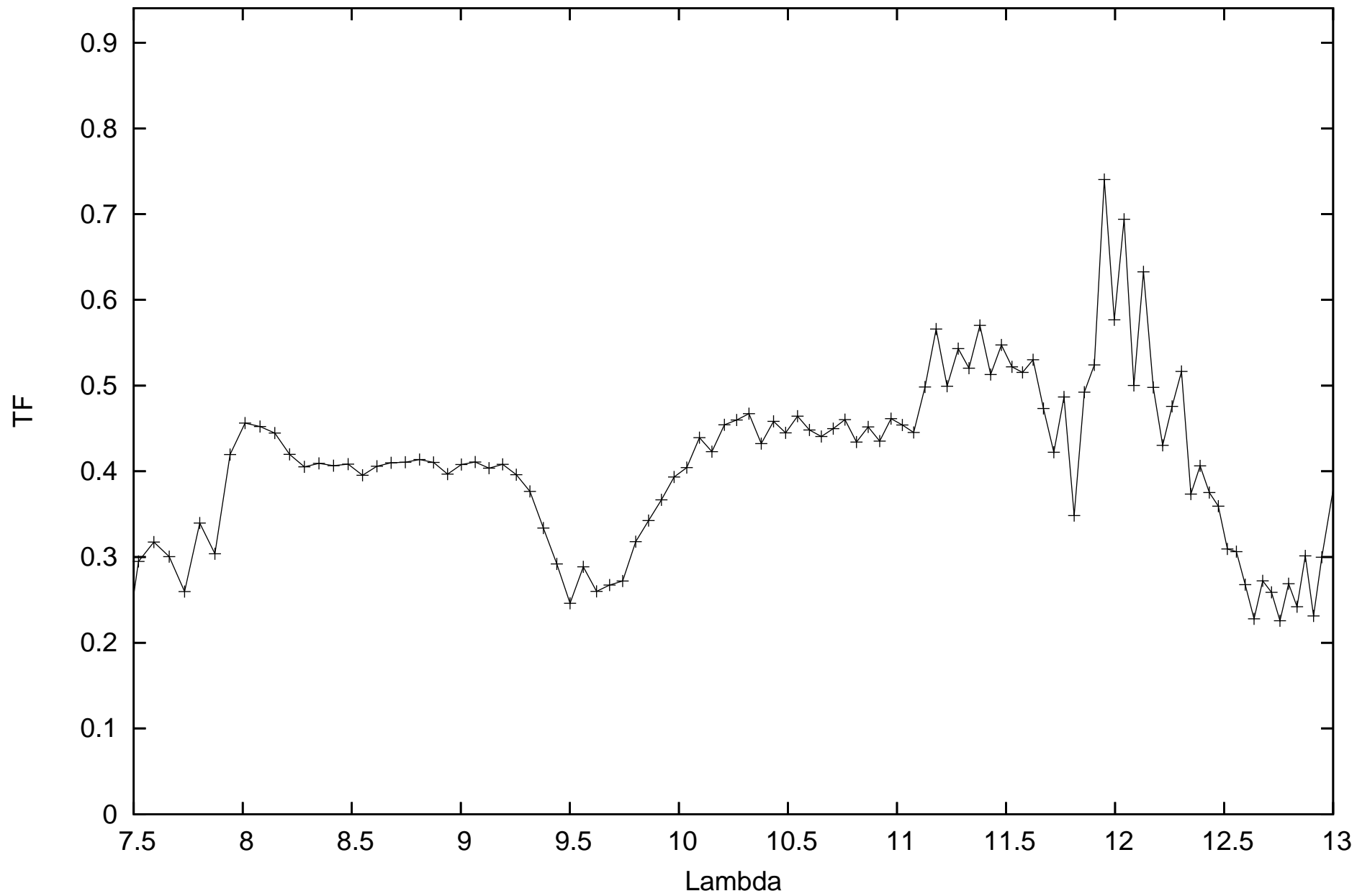
calHD092036_flux0.5_diam4.05_r.MIDI.2009-04-19T02_04_20.000_HIGHSENS
