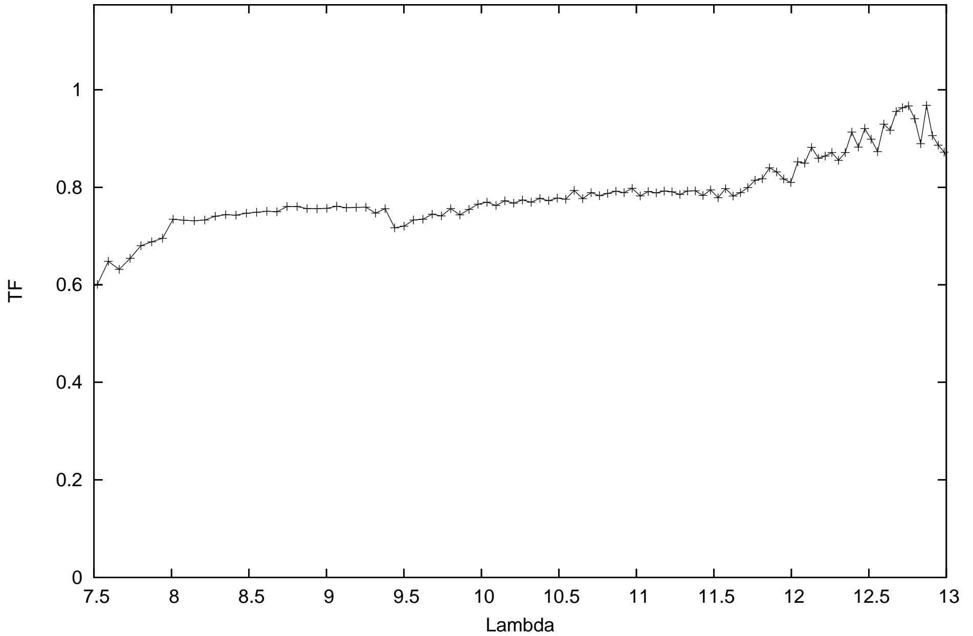
calHD150798_flux-1.4_diam8.91_r.MIDI.2009-04-01T09_45_56.000_HIGHSENS
