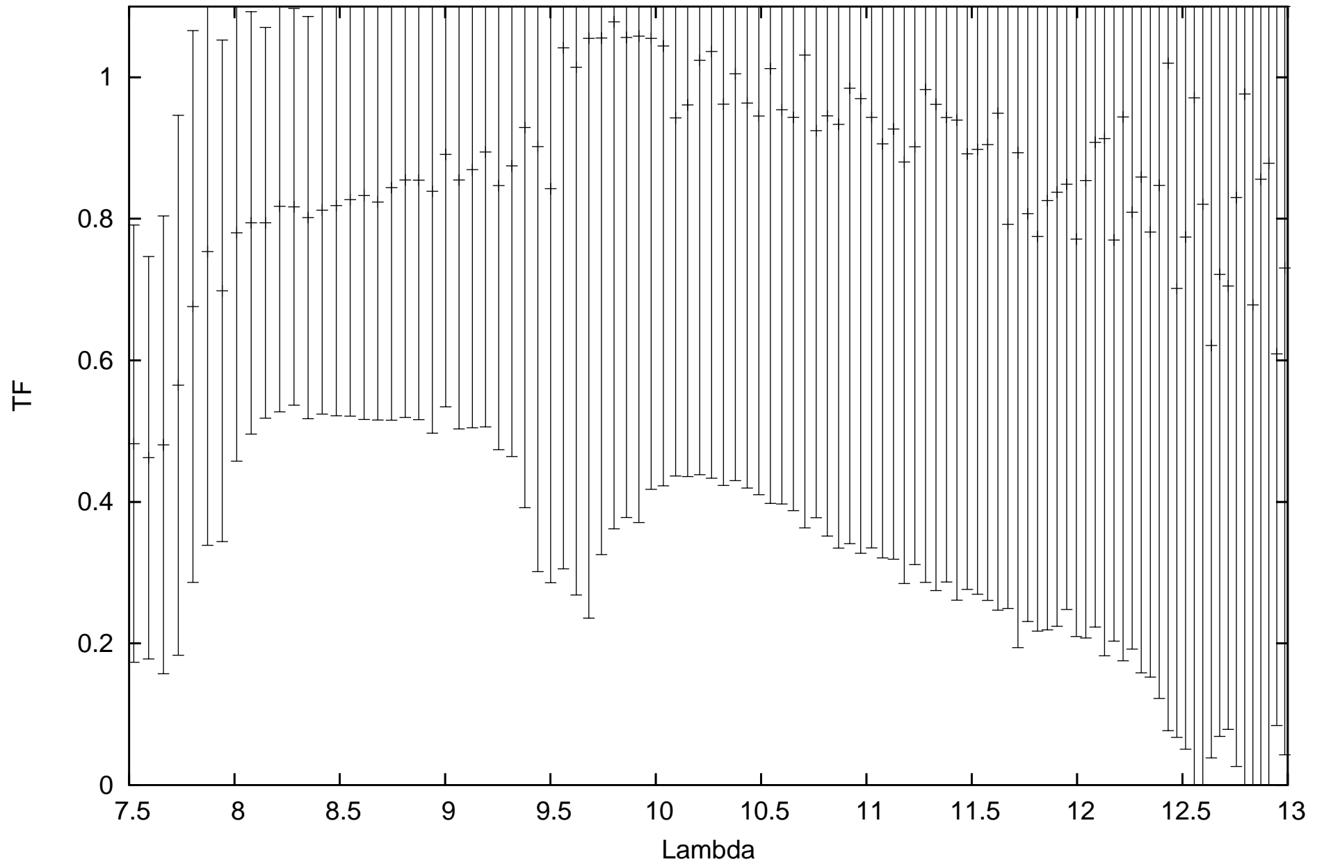
calHD093070_flux0.29_diam4.32_r.MIDI.2009-03-18T03_59_52.000_HIGHSENS
