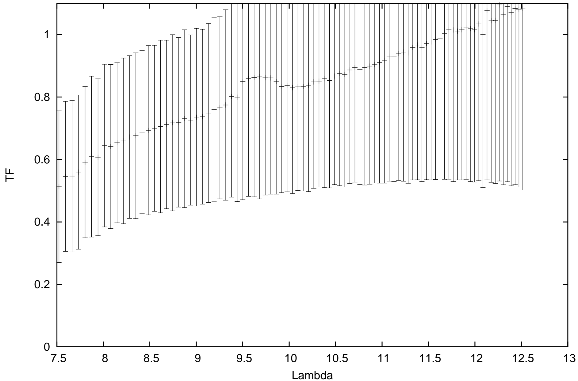
calHD078004_flux1.03_diam2.83_r.MIDI.2009-02-15T04_31_44.000_HIGHSENS
