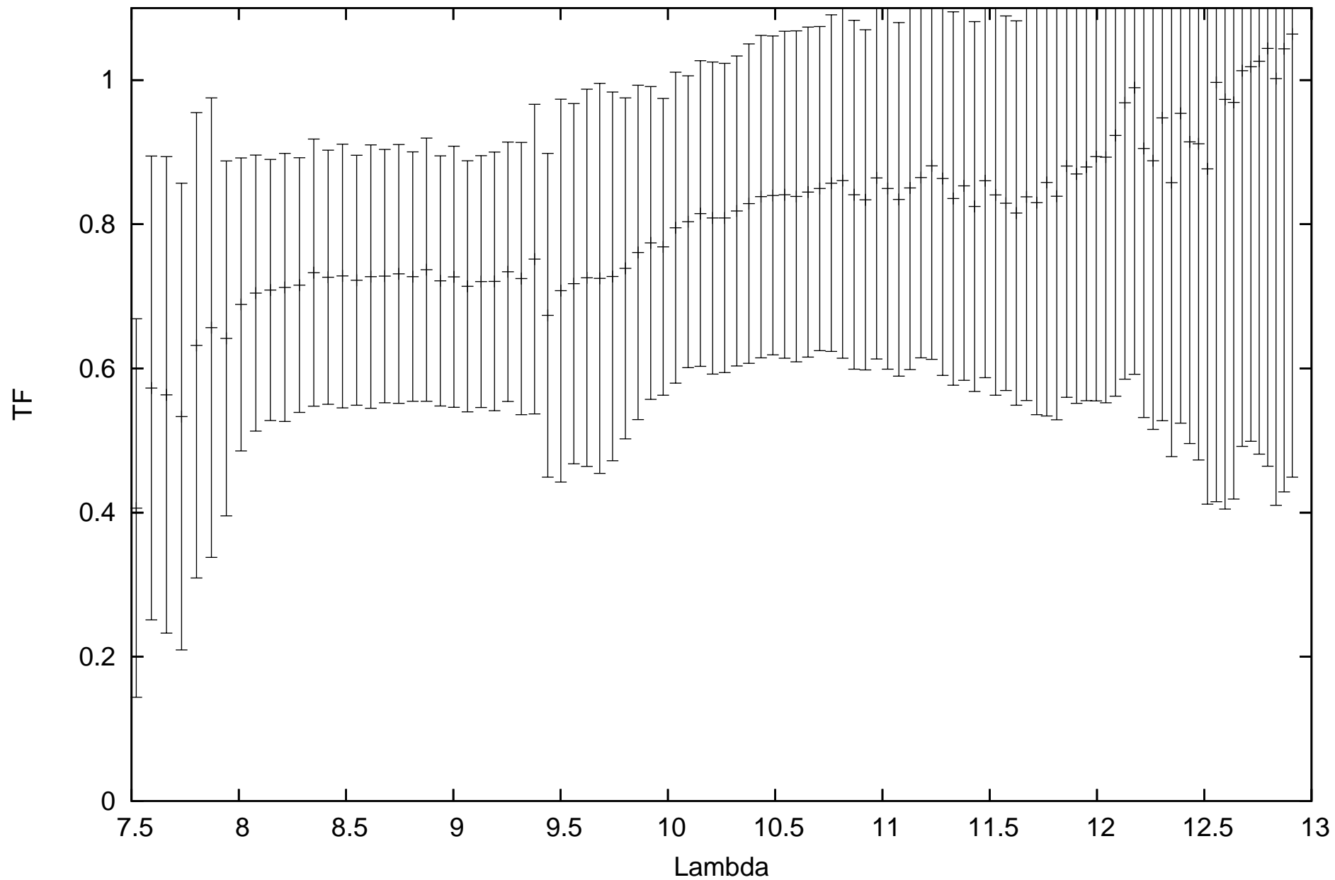
calHD031398_flux-0.85_diam7.1_r.MIDI.2009-01-22T03_17_41.000_HIGHSENS
